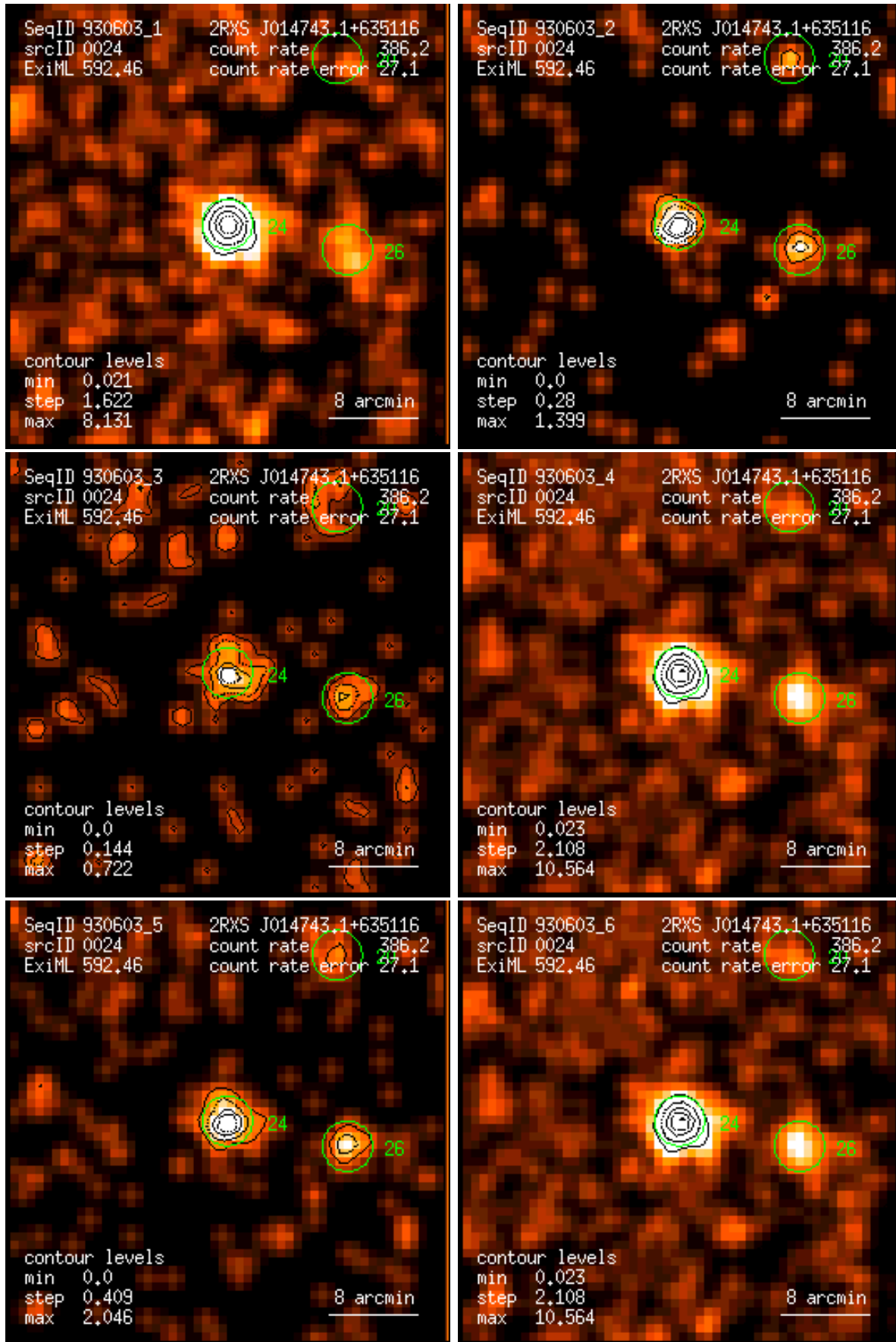
Figure 24: RASS 930603: detection 0024: band rate images, Gaussian filter: (1) PSPC channels 11 – 41, (2) 52 – 90, (3) 91 – 201, (4) 11 – 235, (5) 52 – 201, (6) 11 – 201. Broad band rates in counts/ks. Band rate contour levels in counts/ks/arcmin 2 .
