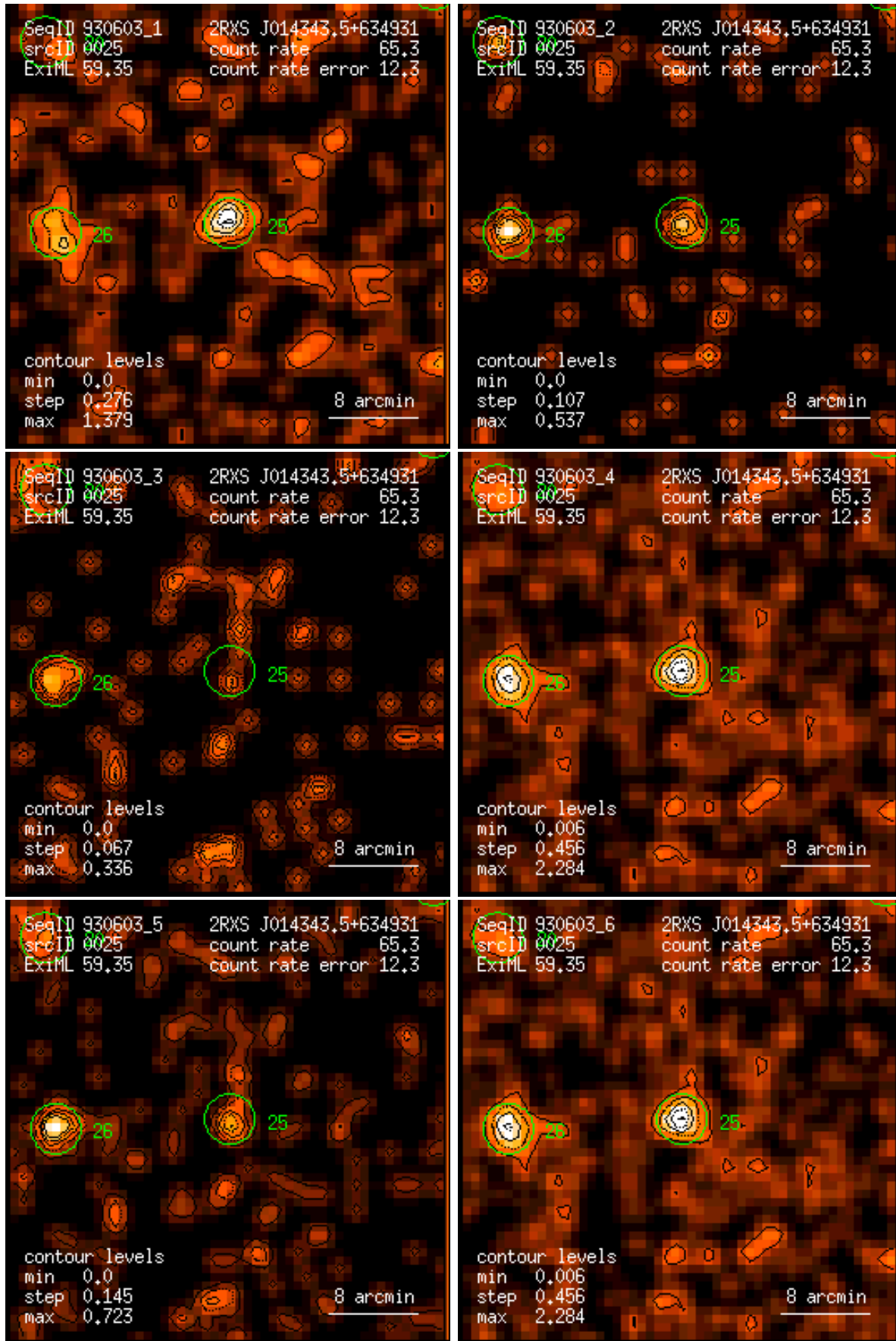
Figure 25: RASS 930603: detection 0025: band rate images, Gaussian filter: (1) PSPC channels 11 – 41, (2) 52 – 90, (3) 91 – 201, (4) 11 – 235, (5) 52 – 201, (6) 11 – 201. Broad band rates in counts/ks. Band rate contour levels in counts/ks/arcmin 2 .
