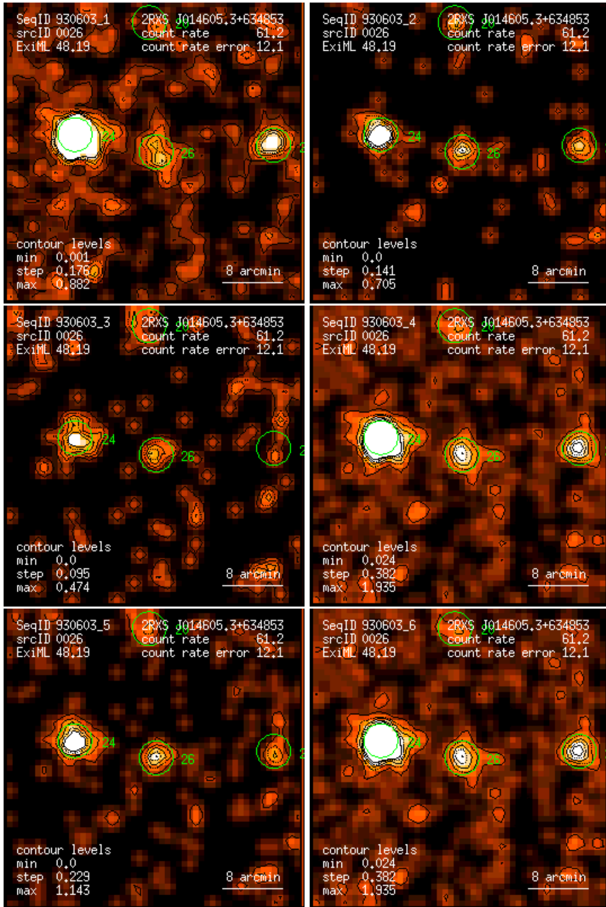
Figure 26: RASS 930603: detection 0026: band rate images, Gaussian filter: (1) PSPC channels 11 – 41, (2) 52 – 90, (3) 91 – 201, (4) 11 – 235, (5) 52 – 201, (6) 11 – 201. Broad band rates in counts/ks. Band rate contour levels in counts/ks/arcmin 2 .
