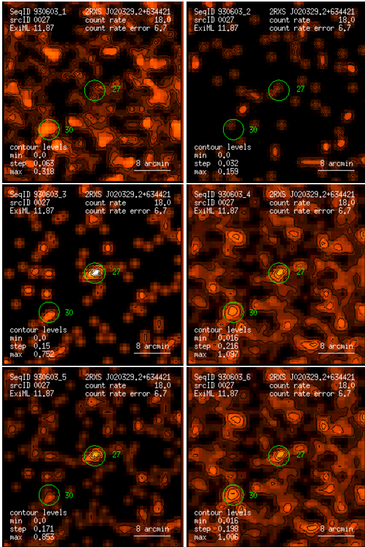
Figure 27: RASS 930603: detection 0027: band rate images, Gaussian filter: (1) PSPC channels 11 – 41, (2) 52 – 90, (3) 91 – 201, (4) 11 – 235, (5) 52 – 201, (6) 11 – 201. Broad band rates in counts/ks. Band rate contour levels in counts/ks/arcmin 2 .
