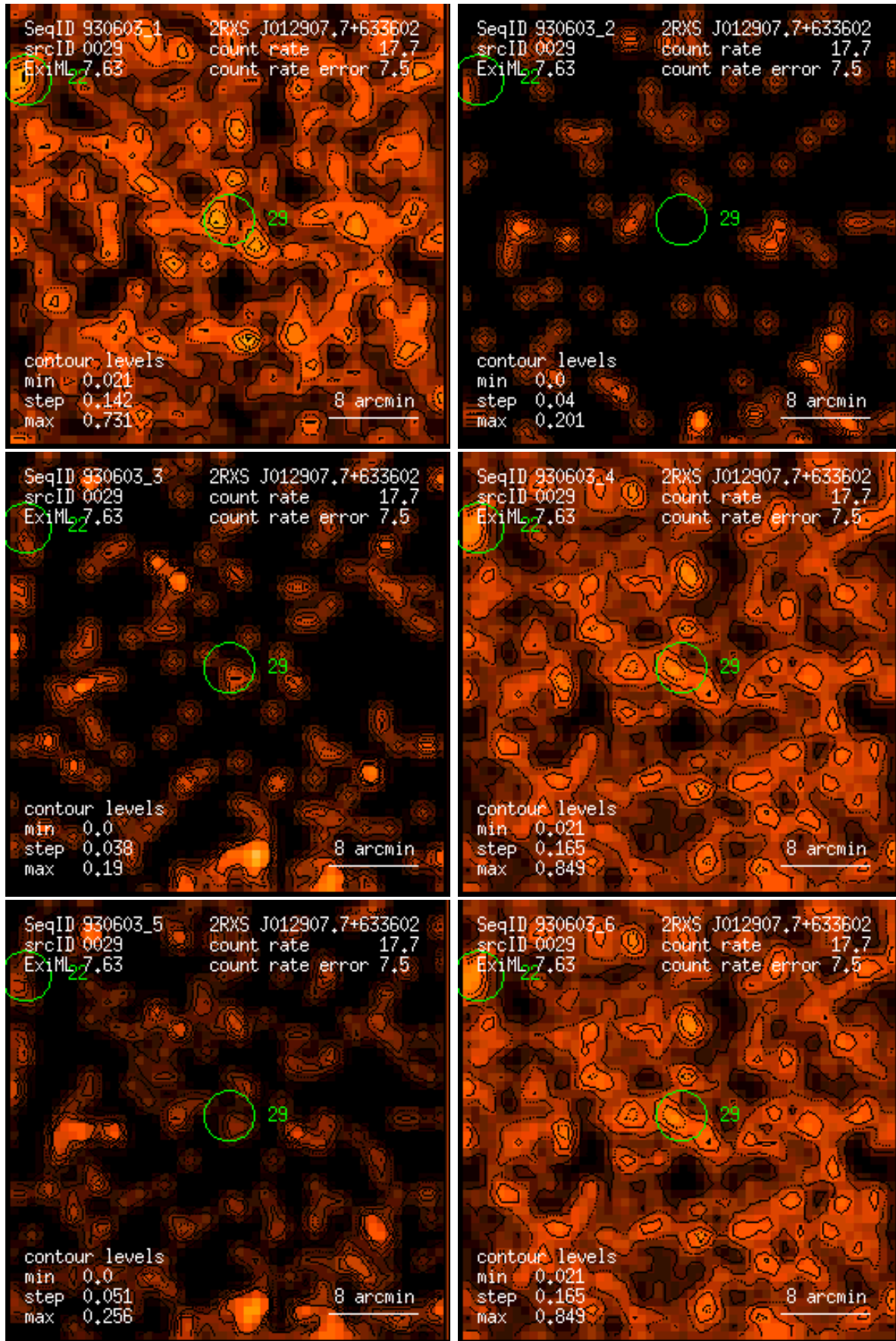
Figure 29: RASS 930603: detection 0029: band rate images, Gaussian filter: (1) PSPC channels 11 – 41, (2) 52 – 90, (3) 91 – 201, (4) 11 – 235, (5) 52 – 201, (6) 11 – 201. Broad band rates in counts/ks. Band rate contour levels in counts/ks/arcmin 2 .
