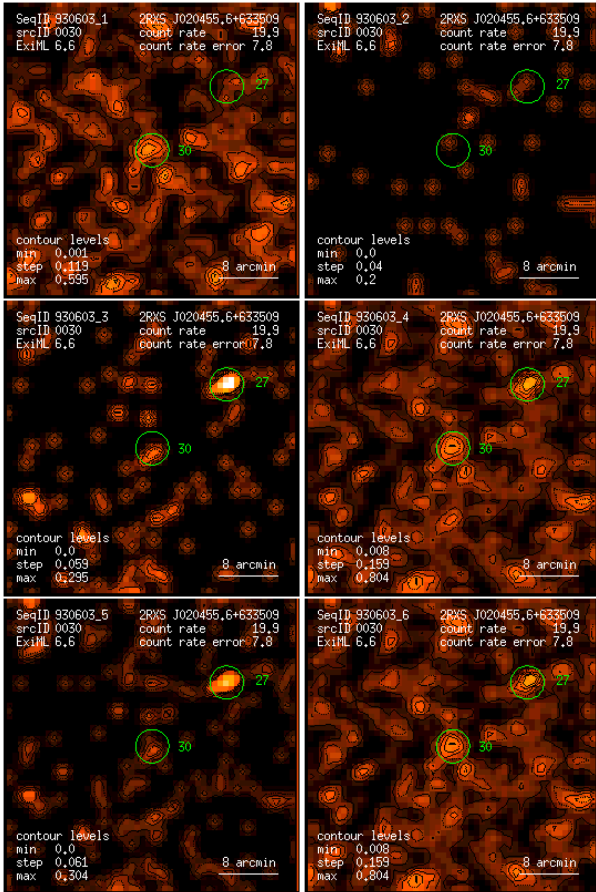
Figure 30: RASS 930603: detection 0030: band rate images, Gaussian filter: (1) PSPC channels 11 – 41, (2) 52 – 90, (3) 91 – 201, (4) 11 – 235, (5) 52 – 201, (6) 11 – 201. Broad band rates in counts/ks. Band rate contour levels in counts/ks/arcmin 2 .
