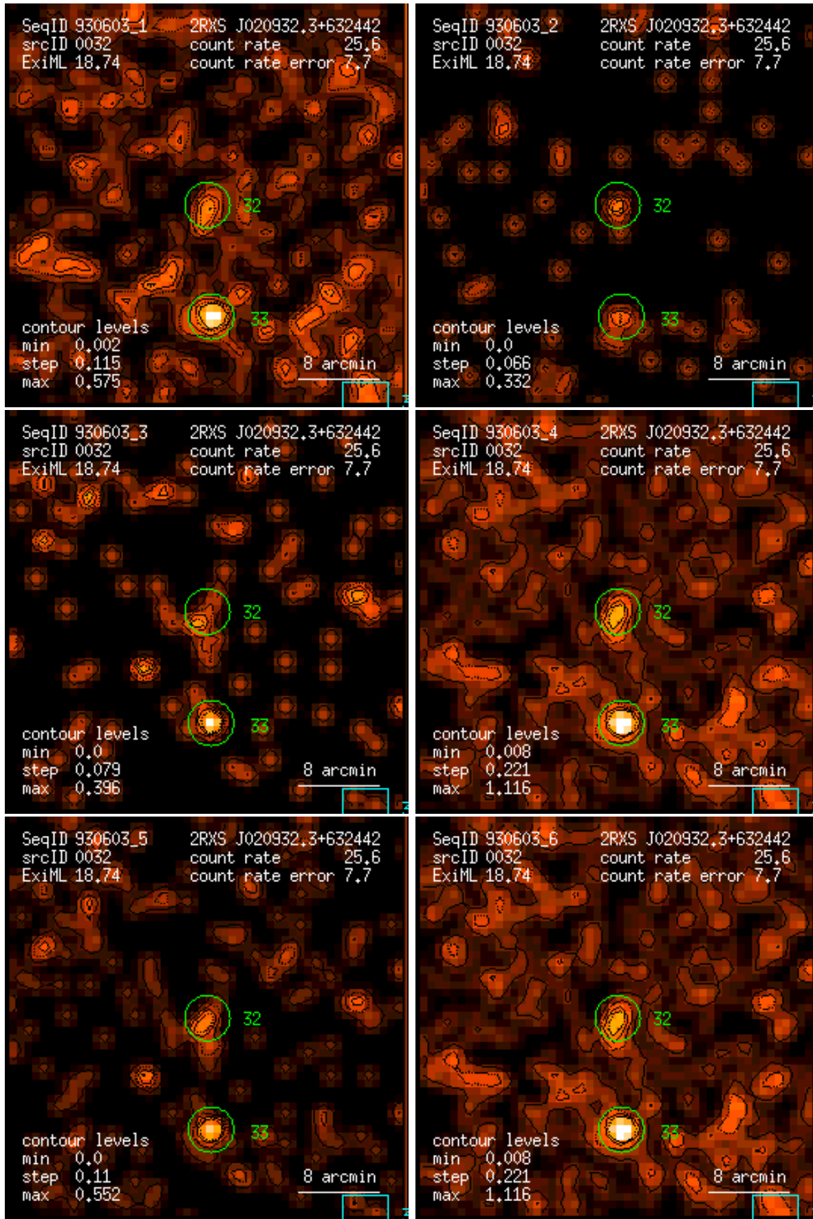
Figure 32: RASS 930603: detection 0032: band rate images, Gaussian filter: (1) PSPC channels 11 – 41, (2) 52 – 90, (3) 91 – 201, (4) 11 – 235, (5) 52 – 201, (6) 11 – 201. Broad band rates in counts/ks. Band rate contour levels in counts/ks/arcmin 2 .
