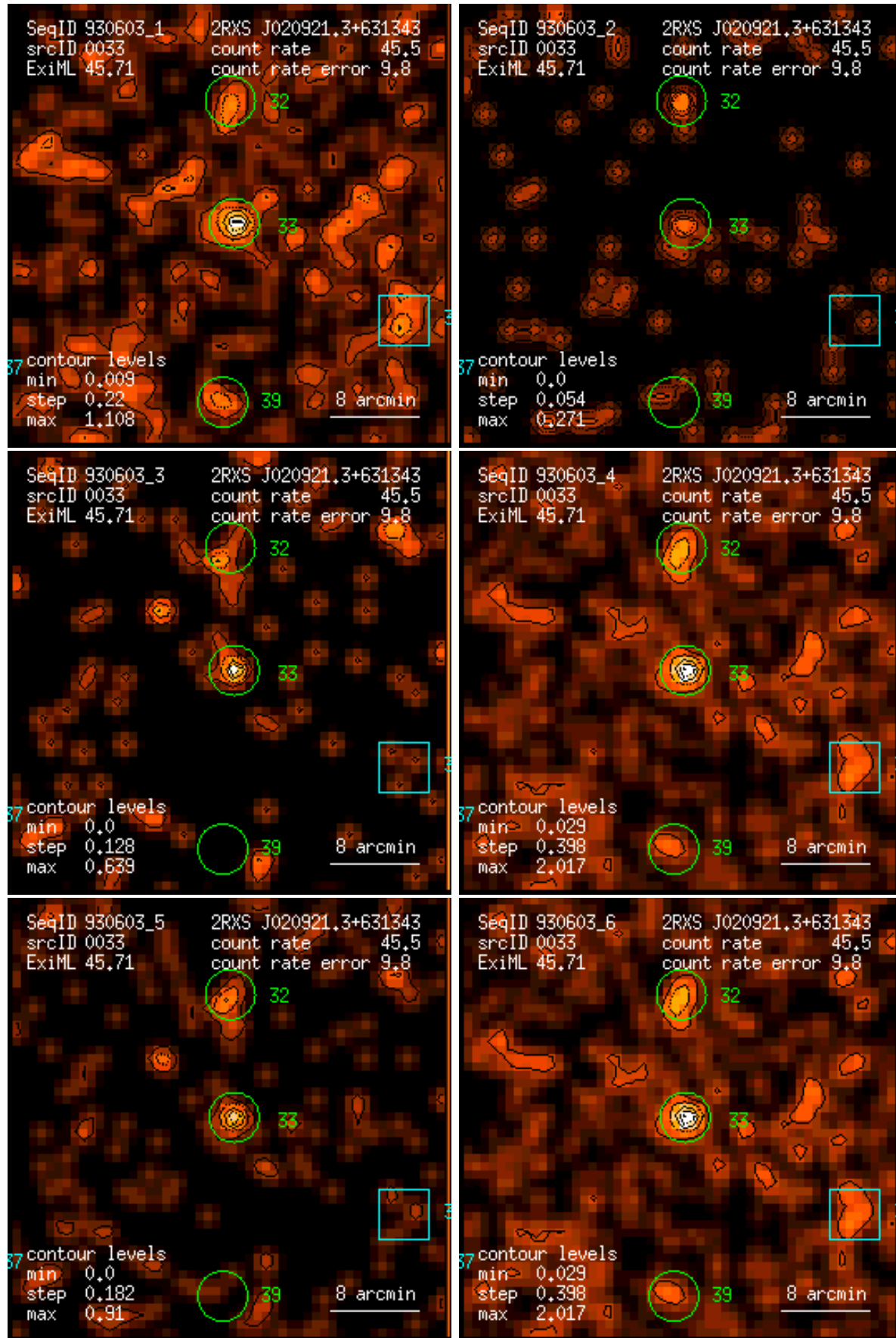
Figure 33: RASS 930603: detection 0033: band rate images, Gaussian filter: (1) PSPC channels 11 – 41, (2) 52 – 90, (3) 91 – 201, (4) 11 – 235, (5) 52 – 201, (6) 11 – 201. Broad band rates in counts/ks. Band rate contour levels in counts/ks/arcmin 2 .
