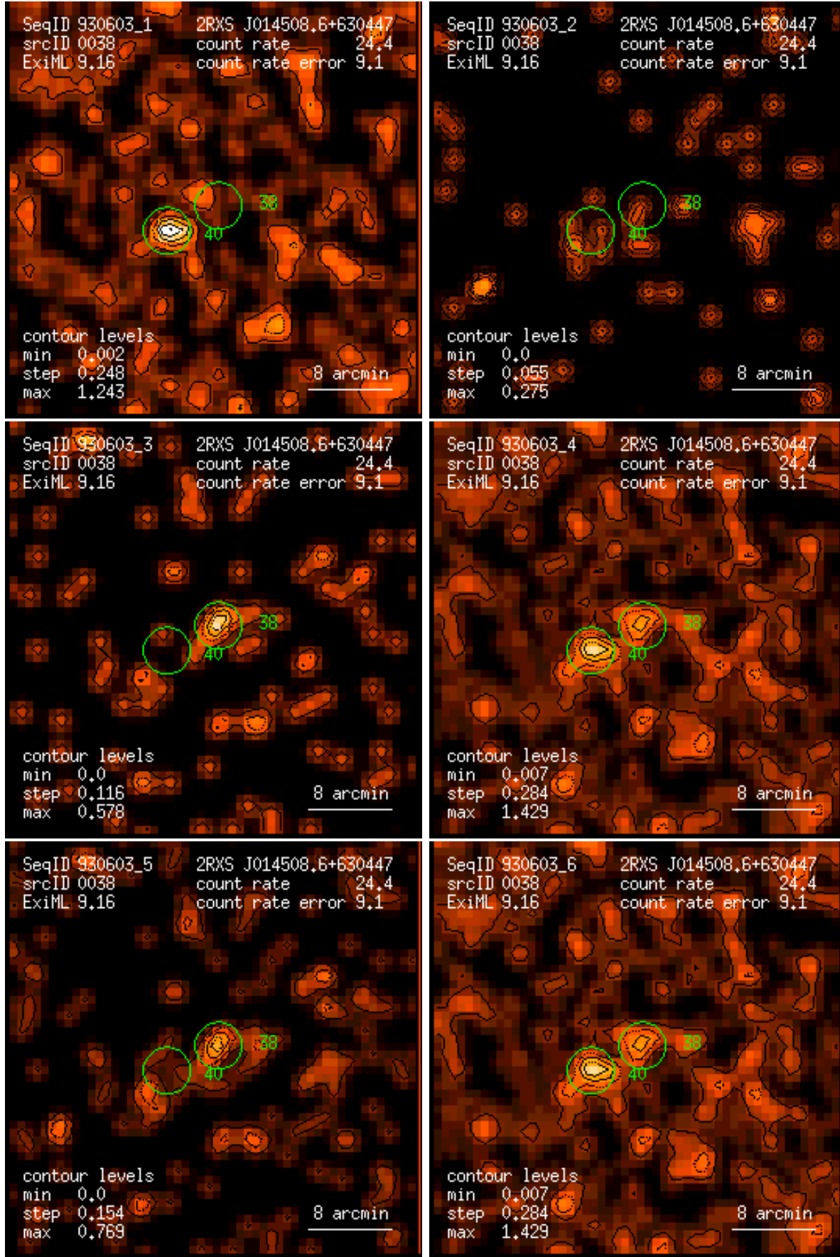
Figure 38: RASS 930603: detection 0038: band rate images, Gaussian filter: (1) PSPC channels 11 – 41, (2) 52 – 90, (3) 91 – 201, (4) 11 – 235, (5) 52 – 201, (6) 11 – 201. Broad band rates in counts/ks. Band rate contour levels in counts/ks/arcmin 2 .
