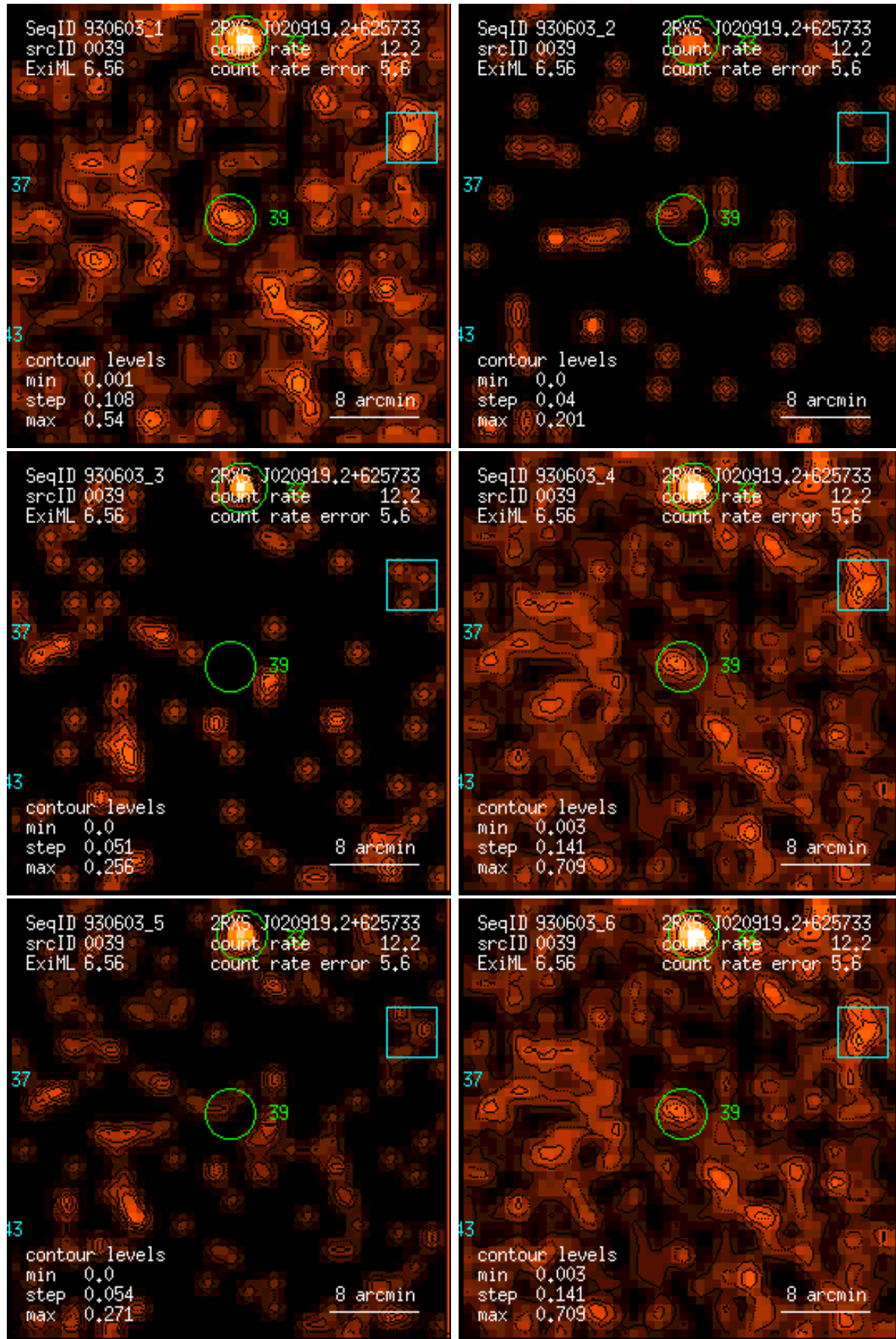
Figure 39: RASS 930603: detection 0039: band rate images, Gaussian filter: (1) PSPP channels 11 – 41, (2) 52 – 90, (3) 91 – 201, (4) 11 – 235, (5) 52 – 201, (6) 11 – 201. Broad band rates in counts/ks. Band rate contour levels in counts/ks/arcmin 2 .
