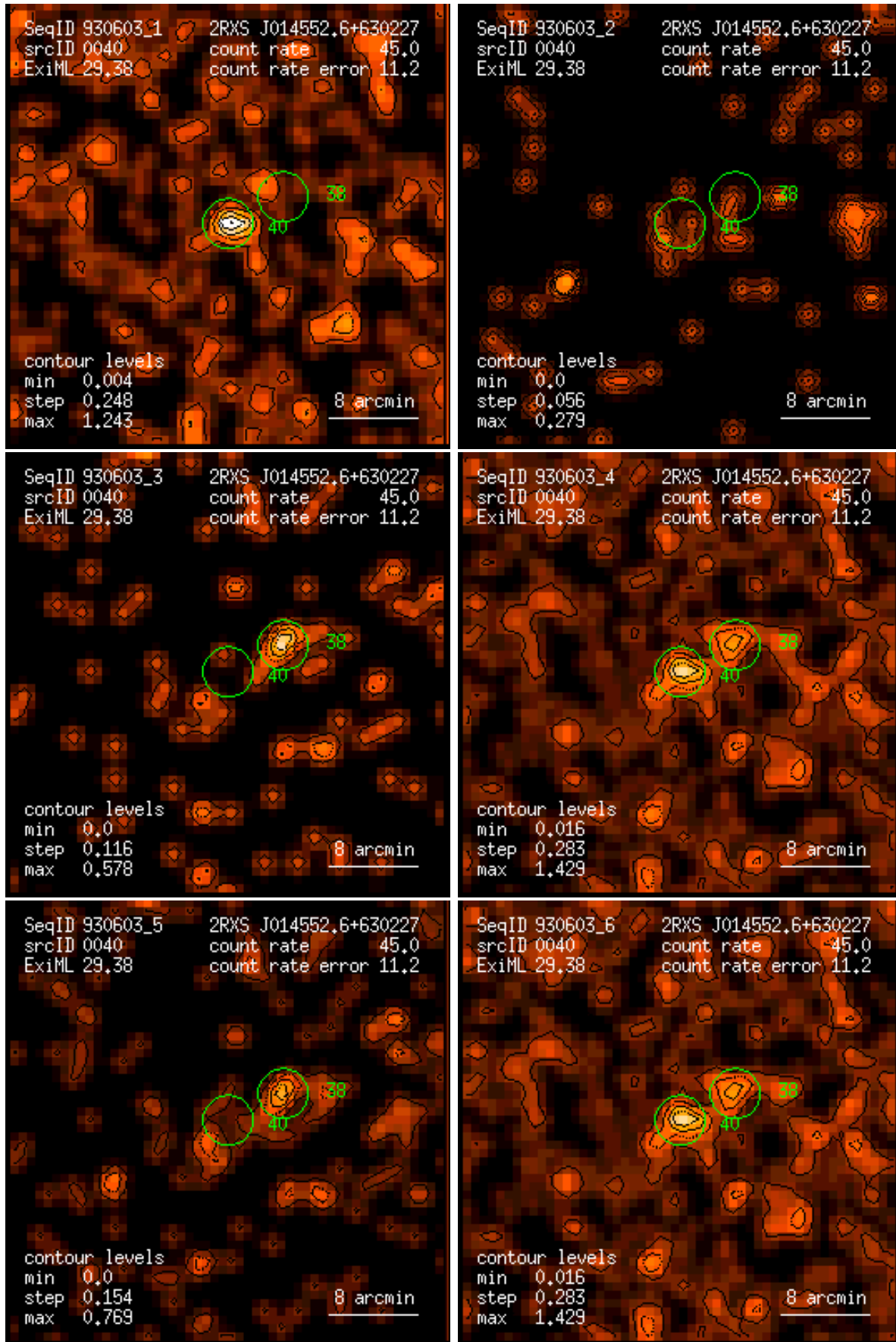
Figure 40: RASS 930603: detection 0040: band rate images, Gaussian filter: (1) PSPC channels 11 – 41, (2) 52 – 90, (3) 91 – 201, (4) 11 – 235, (5) 52 – 201, (6) 11 – 201. Broad band rates in counts/ks. Band rate contour levels in counts/ks/arcmin 2 .
