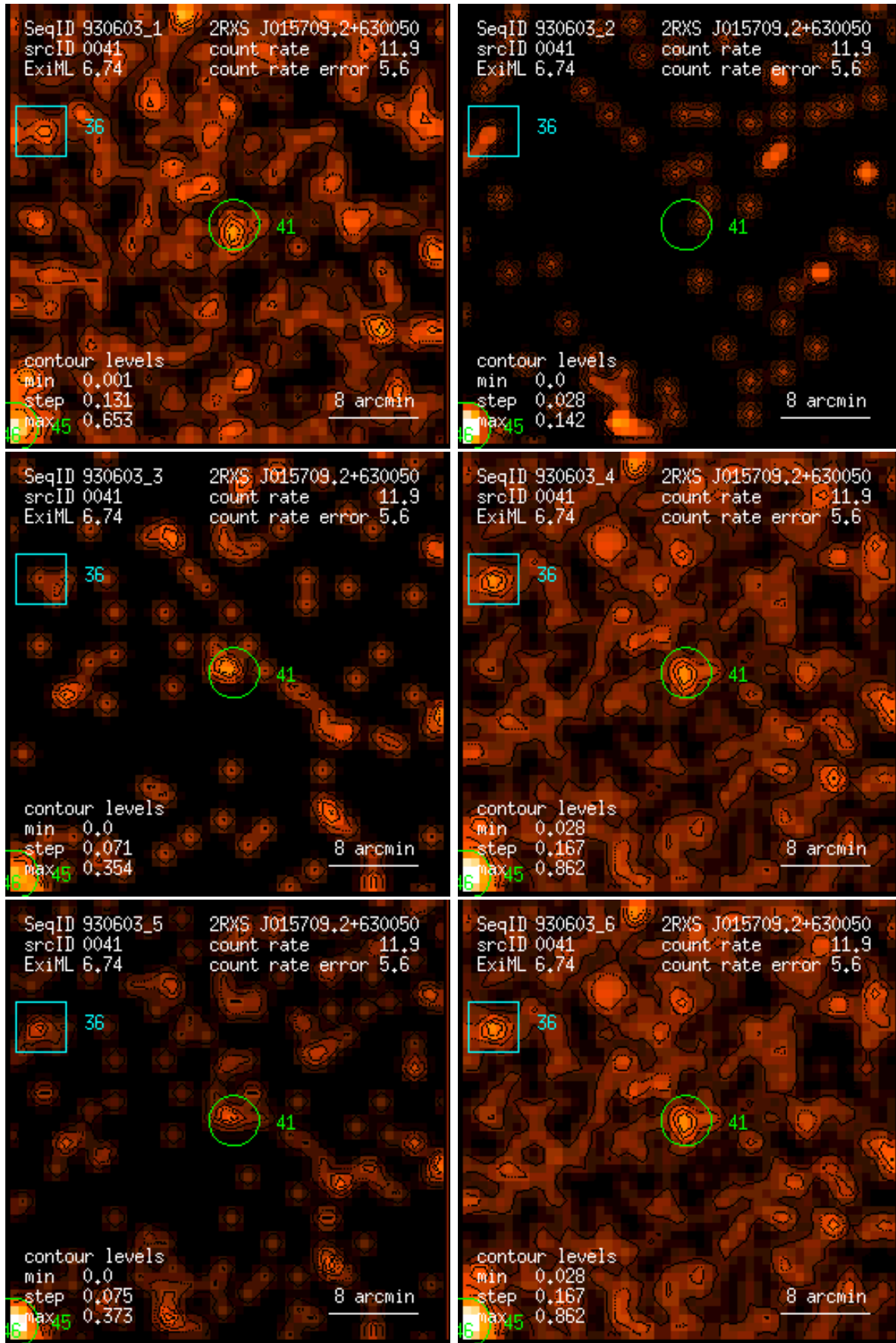
Figure 41: RASS 930603: detection 0041: band rate images, Gaussian filter: (1) PSPC channels 11 – 41, (2) 52 – 90, (3) 91 – 201, (4) 11 – 235, (5) 52 – 201, (6) 11 – 201. Broad band rates in counts/ks. Band rate contour levels in counts/ks/arcmin 2 .
