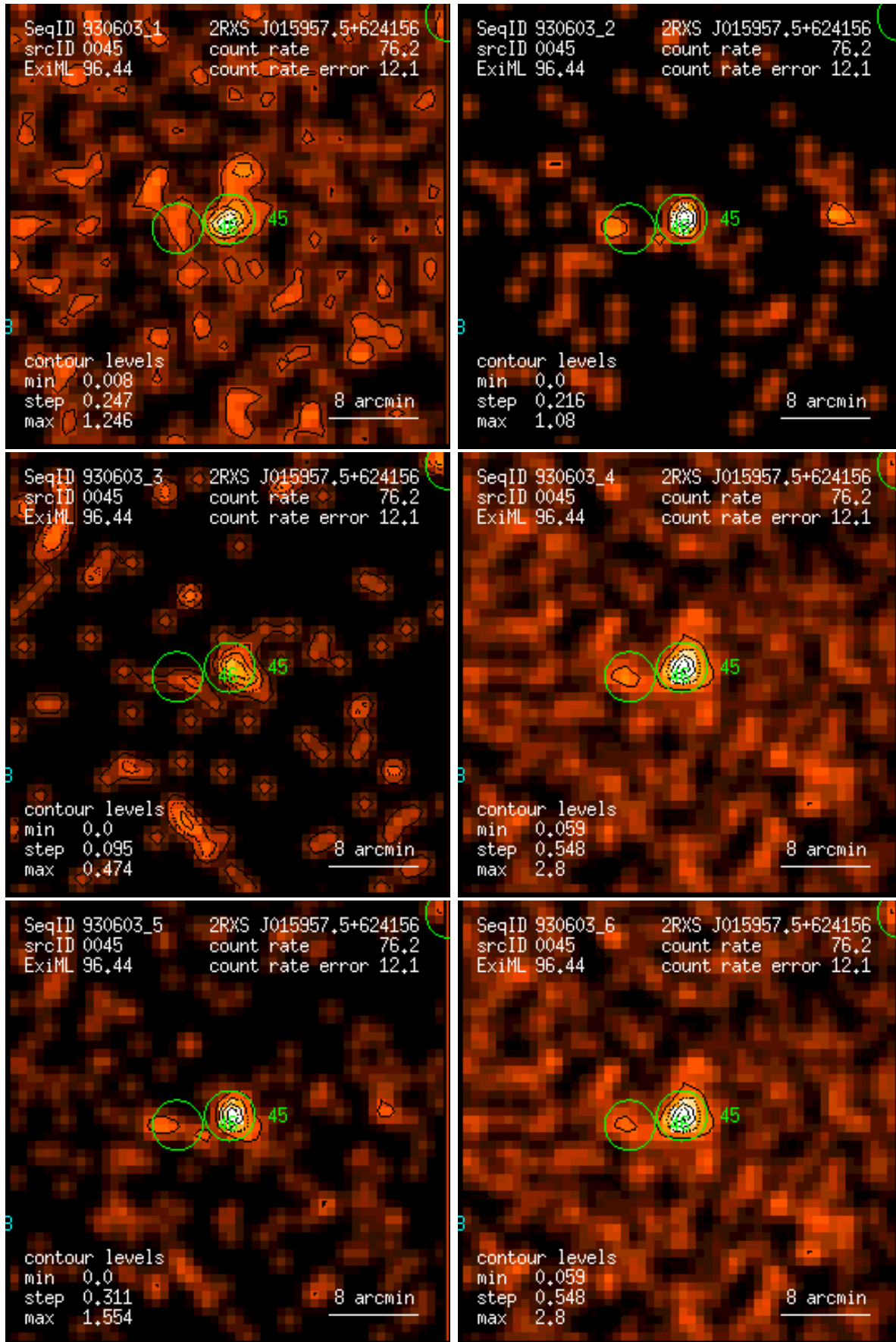
Figure 45: RASS 930603: detection 0045: band rate images, Gaussian filter: (1) PSPC channels 11 – 41, (2) 52 – 90, (3) 91 – 201, (4) 11 – 235, (5) 52 – 201, (6) 11 – 201. Broad band rates in counts/ks. Band rate contour levels in counts/ks/arcmin 2 .
