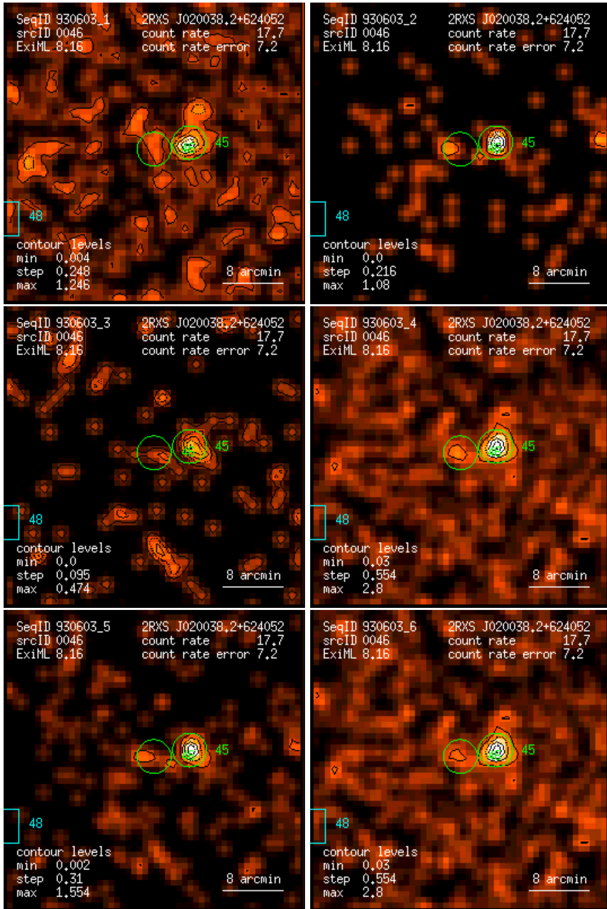
Figure 46: RASS 930603: detection 0046: band rate images, Gaussian filter: (1) PSPC channels 11 – 41, (2) 52 – 90, (3) 91 – 201, (4) 11 – 235, (5) 52 – 201, (6) 11 – 201. Broad band rates in counts/ks. Band rate contour levels in counts/ks/arcmin 2 .
