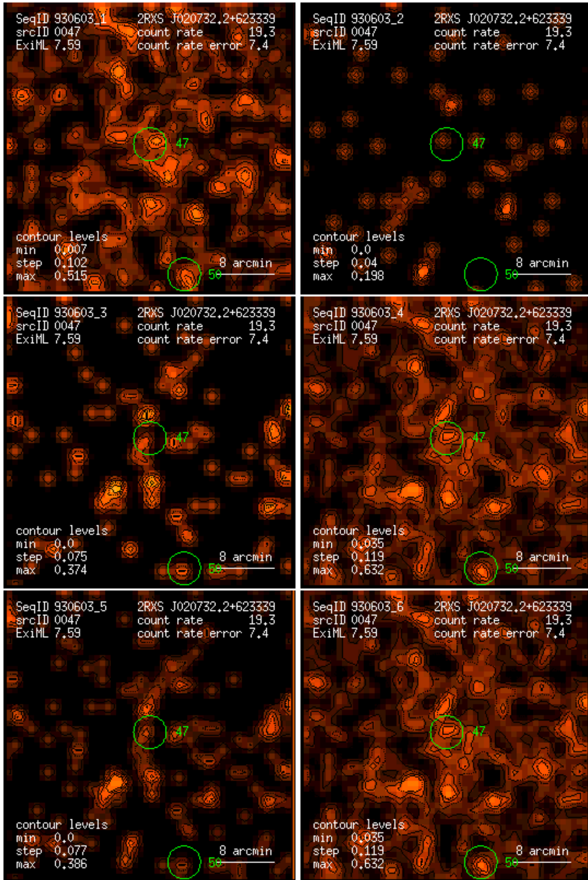
Figure 47: RASS 930603: detection 0047: band rate images, Gaussian filter: (1) PSPC channels 11 – 41, (2) 52 – 90, (3) 91 – 201, (4) 11 – 235, (5) 52 – 201, (6) 11 – 201. Broad band rates in counts/ks. Band rate contour levels in counts/ks/arcmin 2 .
