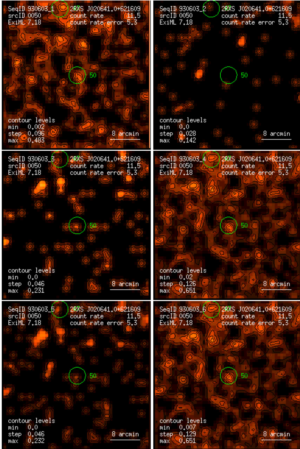
Figure 50: RASS 930603: detection 0050: band rate images, Gaussian filter: (1) PSPC channels 11 – 41, (2) 52 – 90, (3) 91 – 201, (4) 11 – 235, (5) 52 – 201, (6) 11 – 201. Broad band rates in counts/ks. Band rate contour levels in counts/ks/arcmin 2 .
