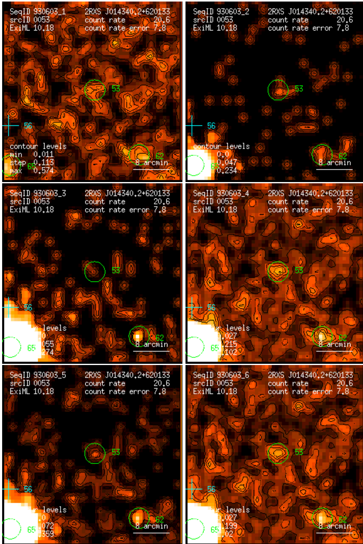
Figure 53: RASS 930603: detection 0053: band rate images, Gaussian filter: (1) PSPC channels 11 – 41, (2) 52 – 90, (3) 91 – 201, (4) 11 – 235, (5) 52 – 201, (6) 11 – 201. Broad band rates in counts/ks. Band rate contour levels in counts/ks/arcmin 2 .
