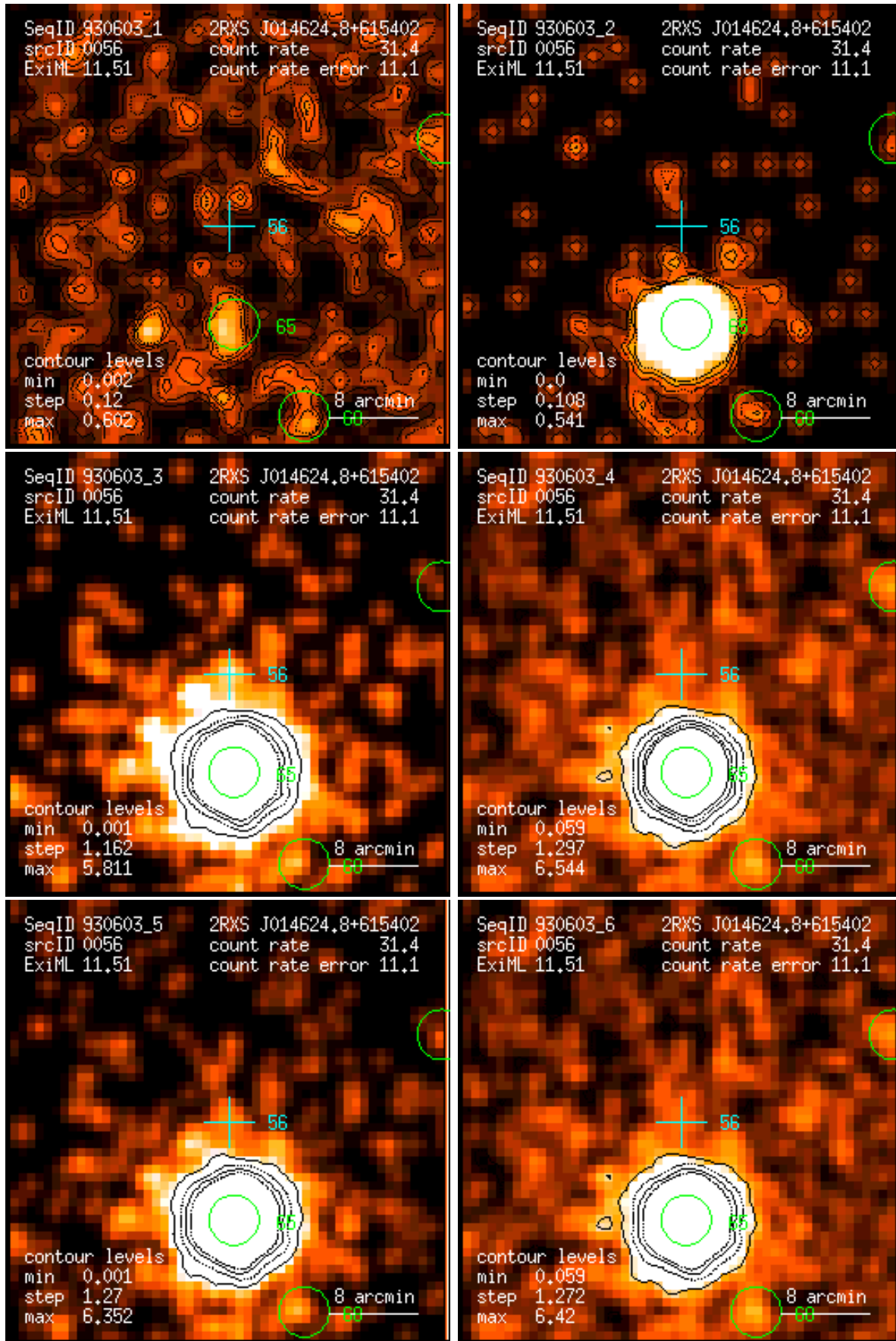
Figure 56: RASS 930603: detection 0056: band rate images, Gaussian filter: (1) PSPC channels 11 – 41, (2) 52 – 90, (3) 91 – 201, (4) 11 – 235, (5) 52 – 201, (6) 11 – 201. Broad band rates in counts/ks. Band rate contour levels in counts/ks/arcmin 2 .
