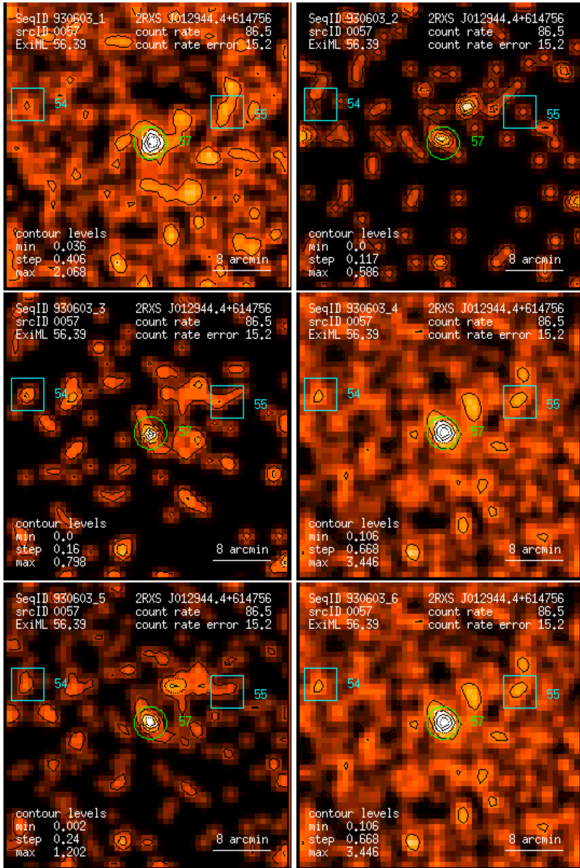
Figure 57: RASS 930603: detection 0057: band rate images, Gaussian filter: (1) PSPC channels 11 – 41, (2) 52 – 90, (3) 91 – 201, (4) 11 – 235, (5) 52 – 201, (6) 11 – 201. Broad band rates in counts/ks. Band rate contour levels in counts/ks/arcmin 2 .
