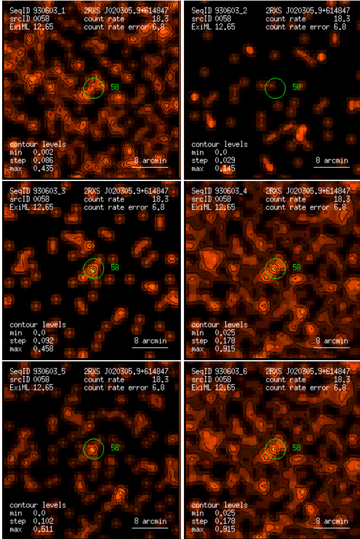
Figure 58: RASS 930603: detection 0058: band rate images, Gaussian filter: (1) PSPC channels 11 – 41, (2) 52 – 90, (3) 91 – 201, (4) 11 – 235, (5) 52 – 201, (6) 11 – 201. Broad band rates in counts/ks. Band rate contour levels in counts/ks/arcmin 2 .
