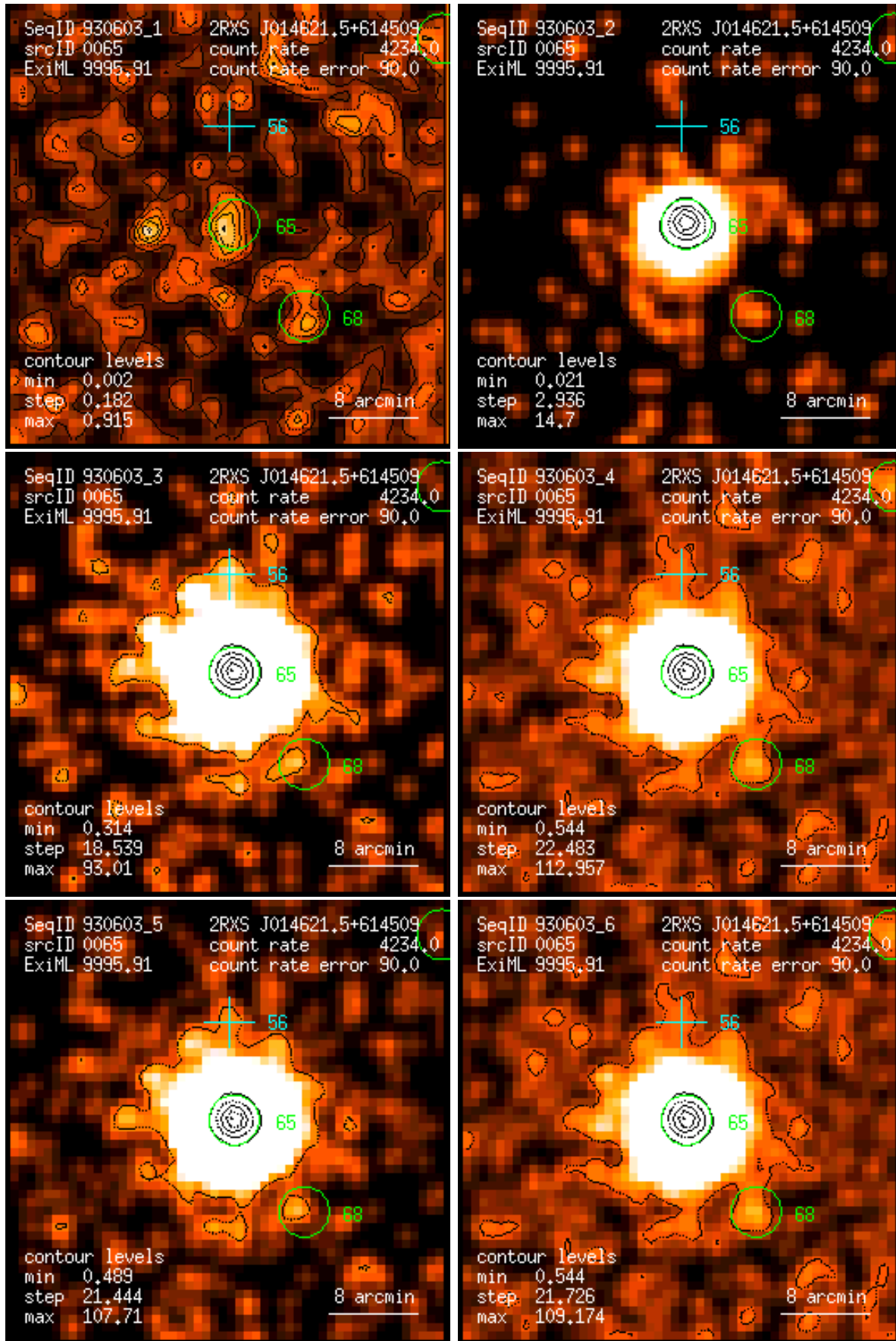
Figure 65: RASS 930603: detection 0065: band rate images, Gaussian filter: (1) PSPC channels 11 – 41, (2) 52 – 90, (3) 91 – 201, (4) 11 – 235, (5) 52 – 201, (6) 11 – 201. Broad band rates in counts/ks. Band rate contour levels in counts/ks/arcmin 2 .
