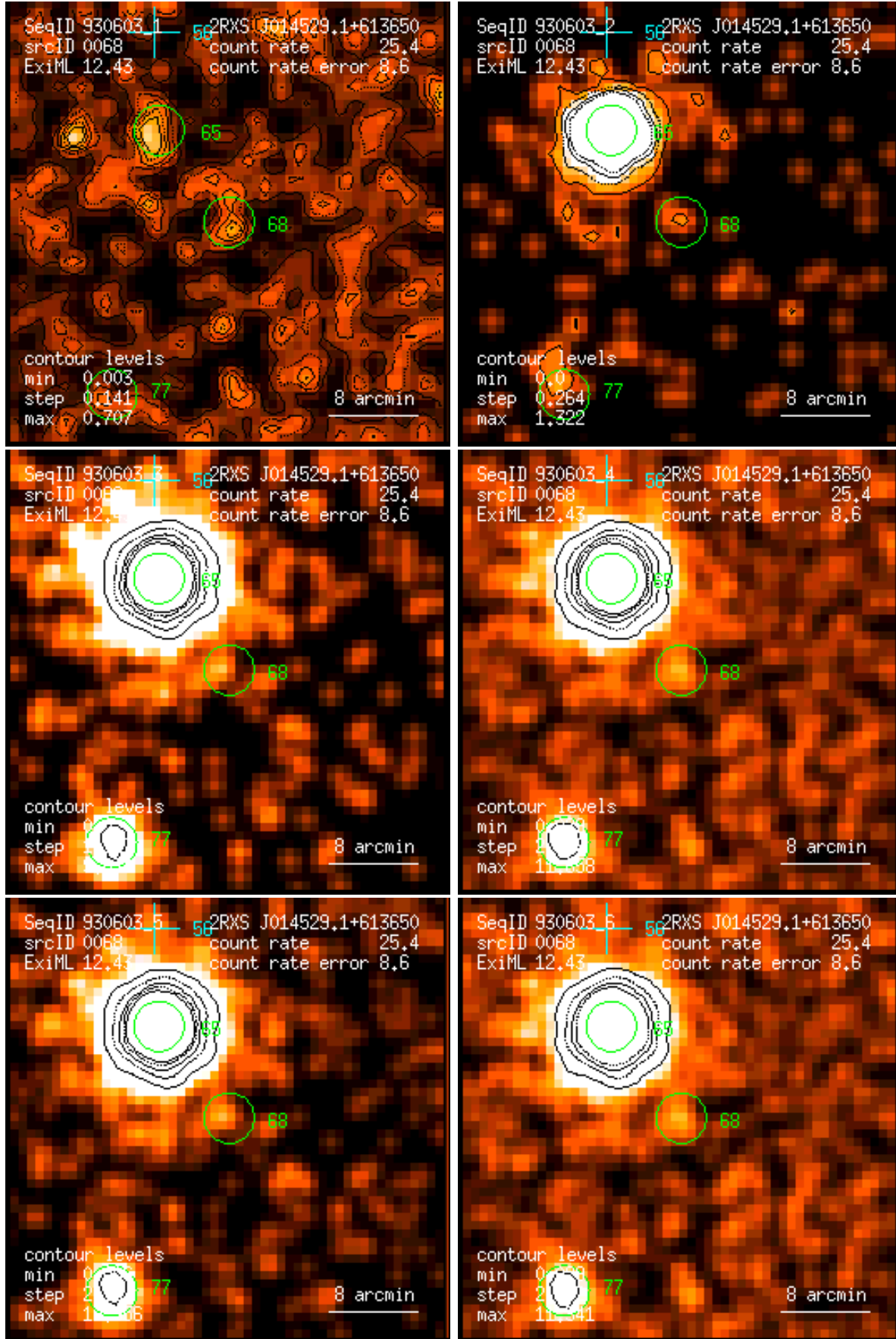
Figure 68: RASS 930603: detection 0068: band rate images, Gaussian filter: (1) PSPC channels 11 – 41, (2) 52 – 90, (3) 91 – 201, (4) 11 – 235, (5) 52 – 201, (6) 11 – 201. Broad band rates in counts/ks. Band rate contour levels in counts/ks/arcmin 2 .
