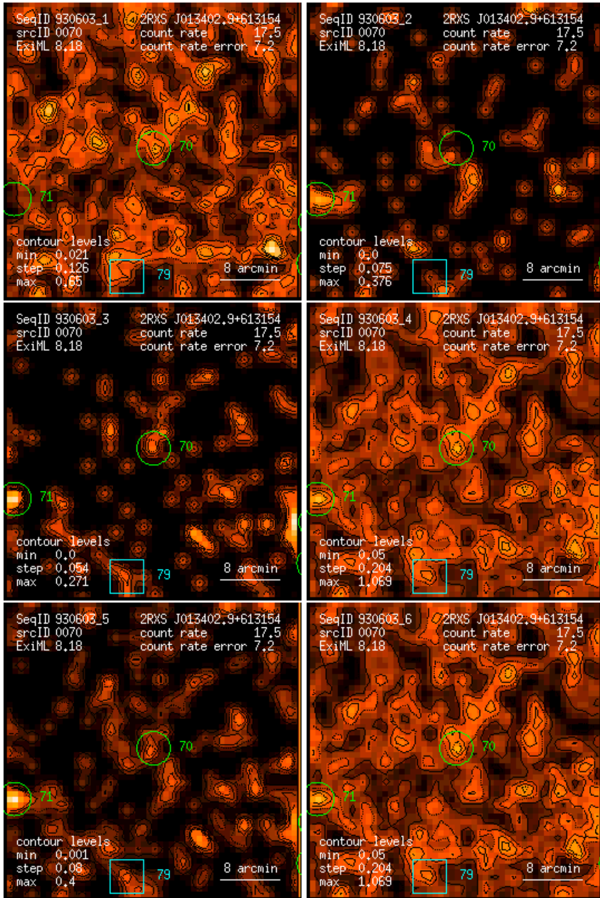
Figure 70: RASS 930603: detection 0070: band rate images, Gaussian filter: (1) PSPC channels 11 – 41, (2) 52 – 90, (3) 91 – 201, (4) 11 – 235, (5) 52 – 201, (6) 11 – 201. Broad band rates in counts/ks. Band rate contour levels in counts/ks/arcmin 2 .
