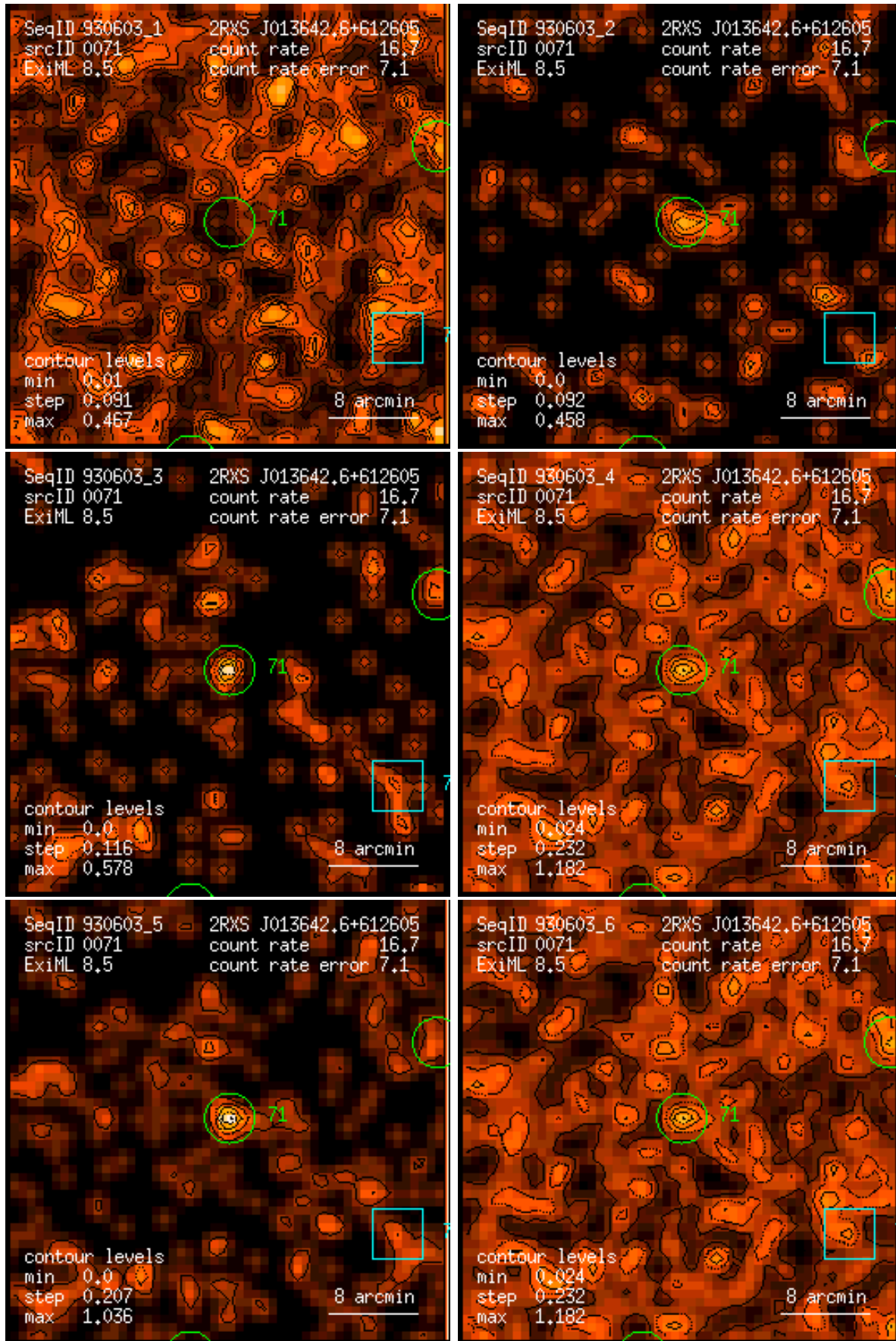
Figure 71: RASS 930603: detection 0071: band rate images, Gaussian filter: (1) PSPC channels 11 – 41, (2) 52 – 90, (3) 91 – 201, (4) 11 – 235, (5) 52 – 201, (6) 11 – 201. Broad band rates in counts/ks. Band rate contour levels in counts/ks/arcmin 2 .
