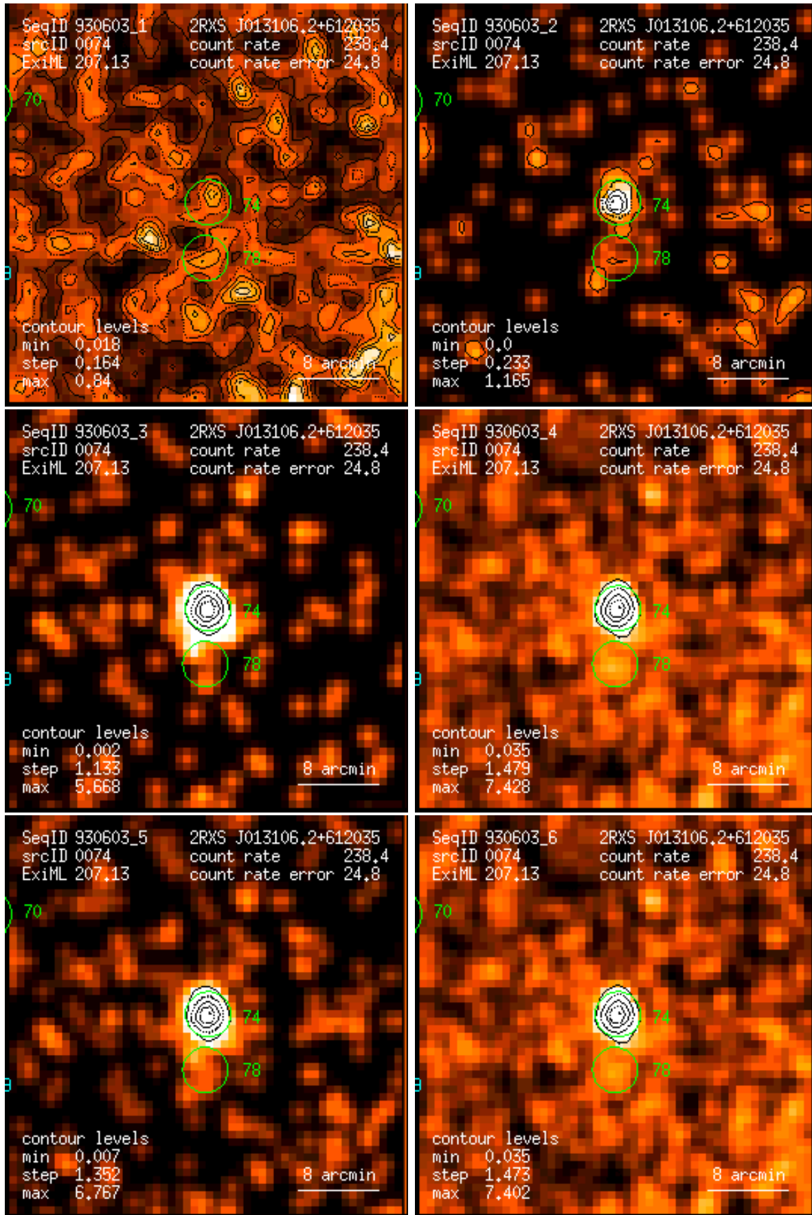
Figure 74: RASS 930603: detection 0074: band rate images, Gaussian filter: (1) PSPC channels 11 – 41, (2) 52 – 90, (3) 91 – 201, (4) 11 – 235, (5) 52 – 201, (6) 11 – 201. Broad band rates in counts/ks. Band rate contour levels in counts/ks/arcmin 2 .
