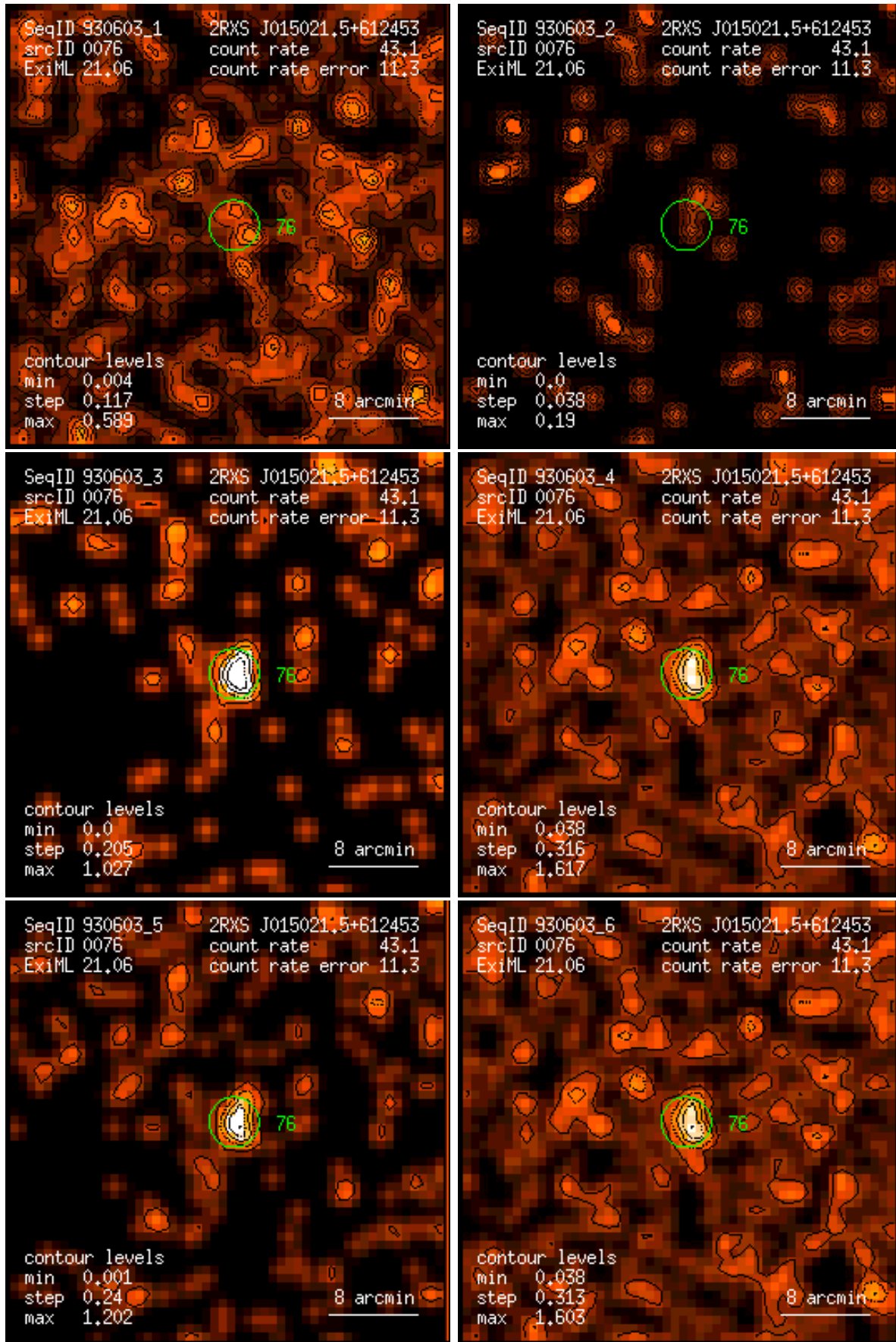
Figure 76: RASS 930603: detection 0076: band rate images, Gaussian filter: (1) PSPC channels 11 – 41, (2) 52 – 90, (3) 91 – 201, (4) 11 – 235, (5) 52 – 201, (6) 11 – 201. Broad band rates in counts/ks. Band rate contour levels in counts/ks/arcmin 2 .
