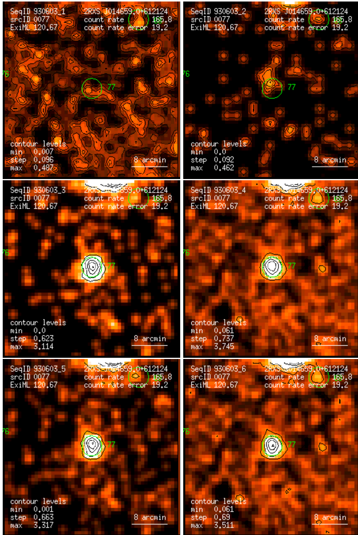
Figure 77: RASS 930603: detection 0077: band rate images, Gaussian filter: (1) PSPC channels 11 – 41, (2) 52 – 90, (3) 91 – 201, (4) 11 – 235, (5) 52 – 201, (6) 11 – 201. Broad band rates in counts/ks. Band rate contour levels in counts/ks/arcmin 2 .
