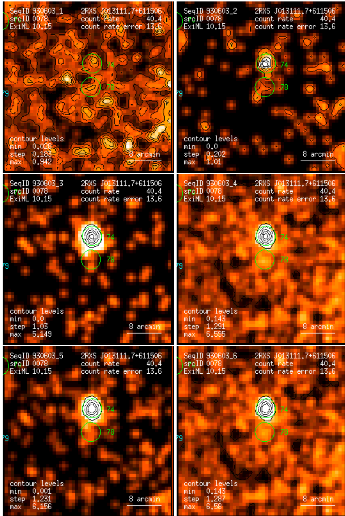
Figure 78: RASS 930603: detection 0078: band rate images, Gaussian filter: (1) PSPC channels 11 – 41, (2) 52 – 90, (3) 91 – 201, (4) 11 – 235, (5) 52 – 201, (6) 11 – 201. Broad band rates in counts/ks. Band rate contour levels in counts/ks/arcmin 2 .
