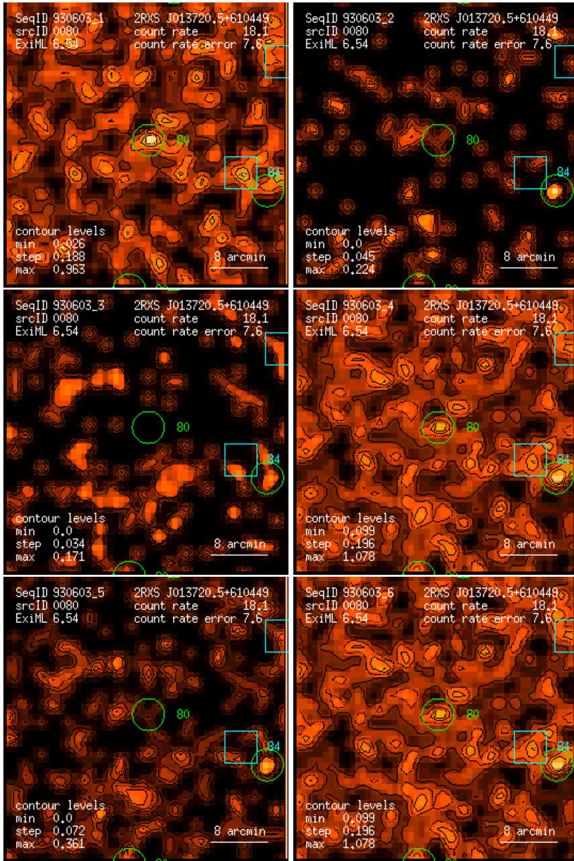
Figure 80: RASS 930603: detection 0080: band rate images, Gaussian filter: (1) PSPC channels 11 – 41, (2) 52 – 90, (3) 91 – 201, (4) 11 – 235, (5) 52 – 201, (6) 11 – 201. Broad band rates in counts/ks. Band rate contour levels in counts/ks/arcmin 2 .
