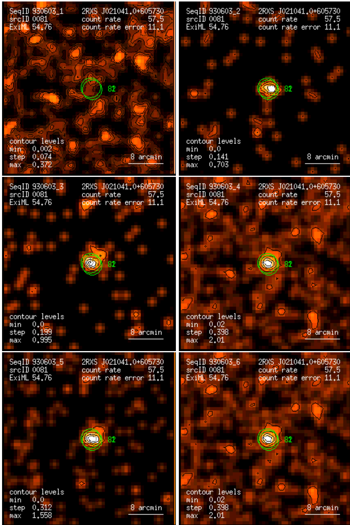
Figure 81: RASS 930603: detection 0081: band rate images, Gaussian filter: (1) PSPC channels 11 – 41, (2) 52 – 90, (3) 91 – 201, (4) 11 – 235, (5) 52 – 201, (6) 11 – 201. Broad band rates in counts/ks. Band rate contour levels in counts/ks/arcmin 2 .
