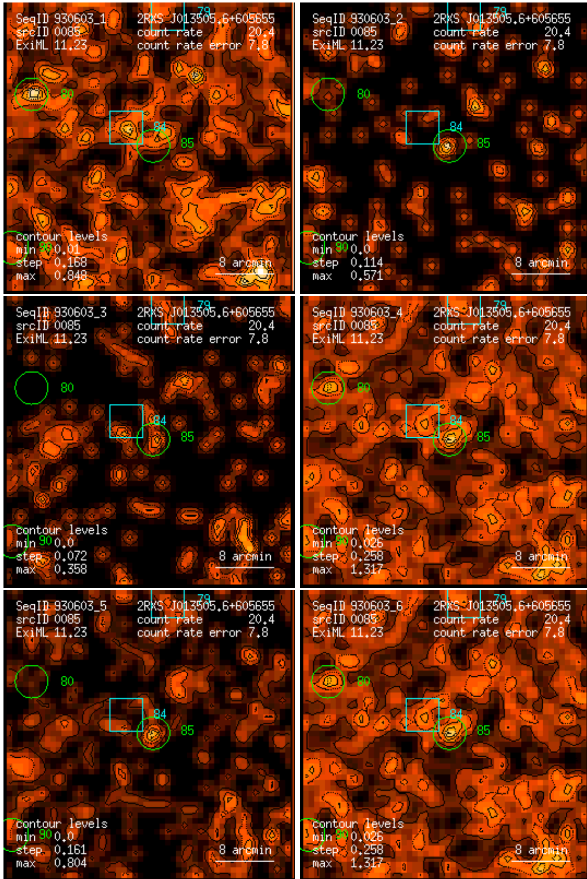
Figure 85: RASS 930603: detection 0085: band rate images, Gaussian filter: (1) PSPC channels 11 – 41, (2) 52 – 90, (3) 91 – 201, (4) 11 – 235, (5) 52 – 201, (6) 11 – 201. Broad band rates in counts/ks. Band rate contour levels in counts/ks/arcmin 2 .
