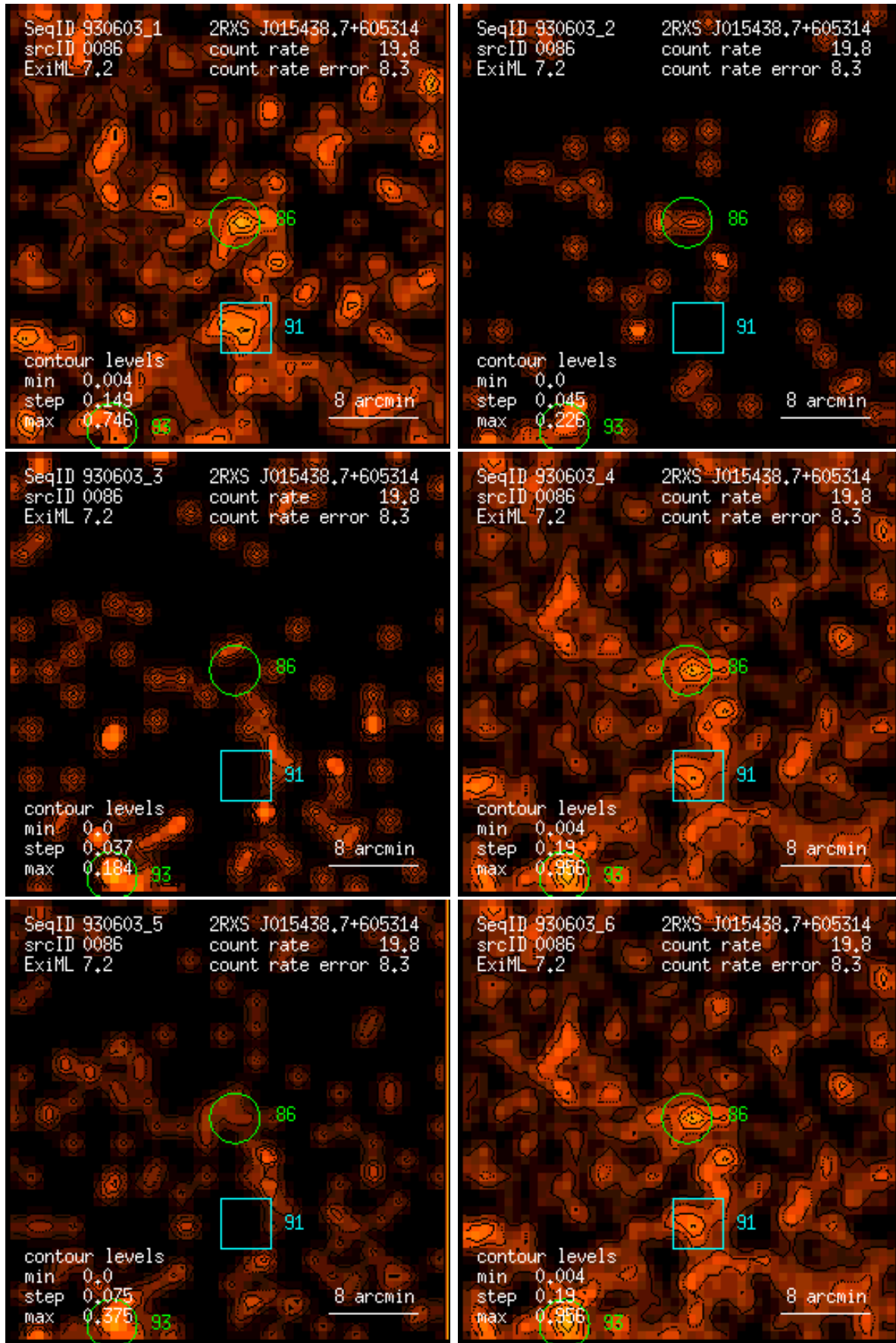
Figure 86: RASS 930603: detection 0086: band rate images, Gaussian filter: (1) PSPC channels 11 – 41, (2) 52 – 90, (3) 91 – 201, (4) 11 – 235, (5) 52 – 201, (6) 11 – 201. Broad band rates in counts/ks. Band rate contour levels in counts/ks/arcmin 2 .
