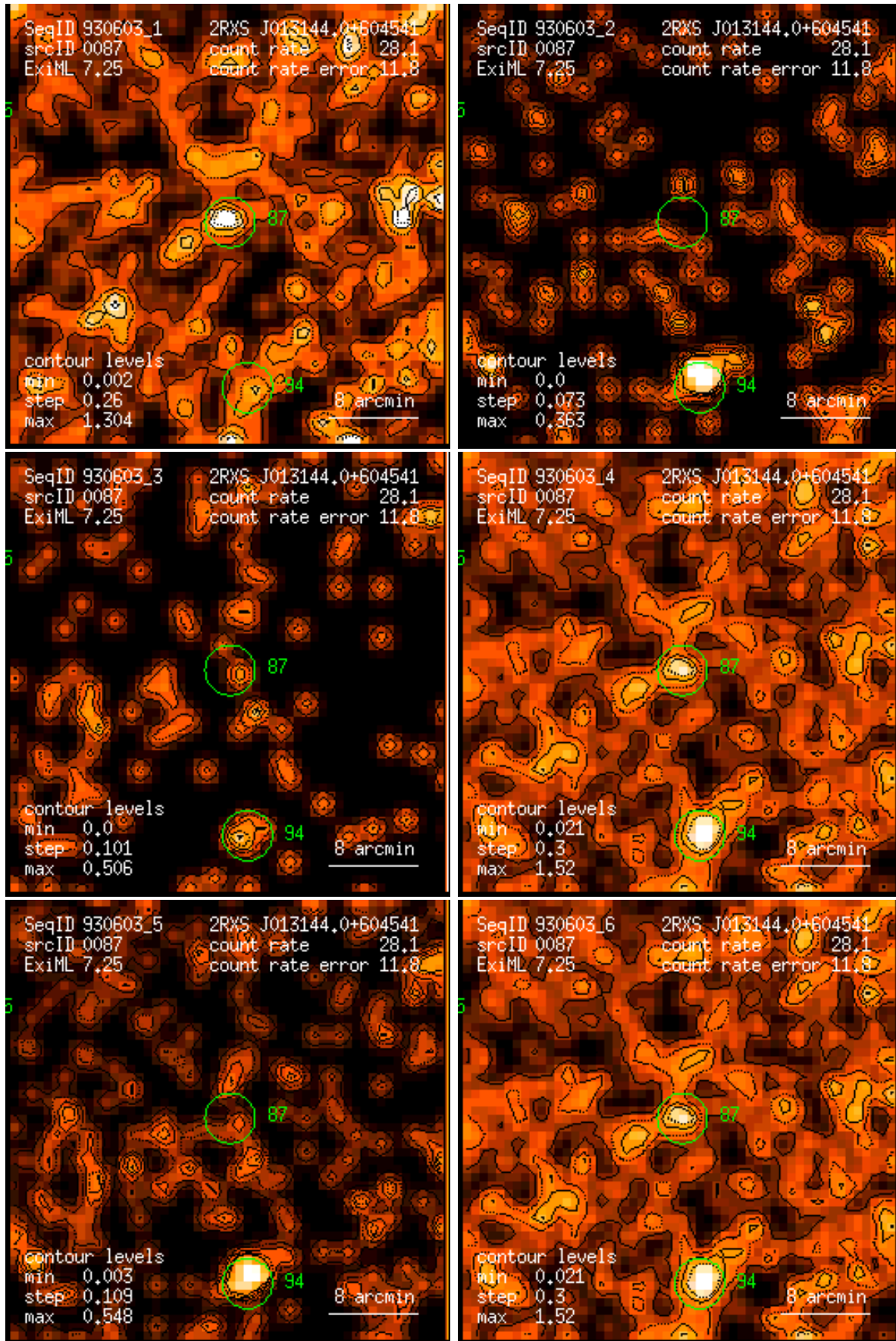
Figure 87: RASS 930603: detection 0087: band rate images, Gaussian filter: (1) PSPC channels 11 – 41, (2) 52 – 90, (3) 91 – 201, (4) 11 – 235, (5) 52 – 201, (6) 11 – 201. Broad band rates in counts/ks. Band rate contour levels in counts/ks/arcmin 2 .
