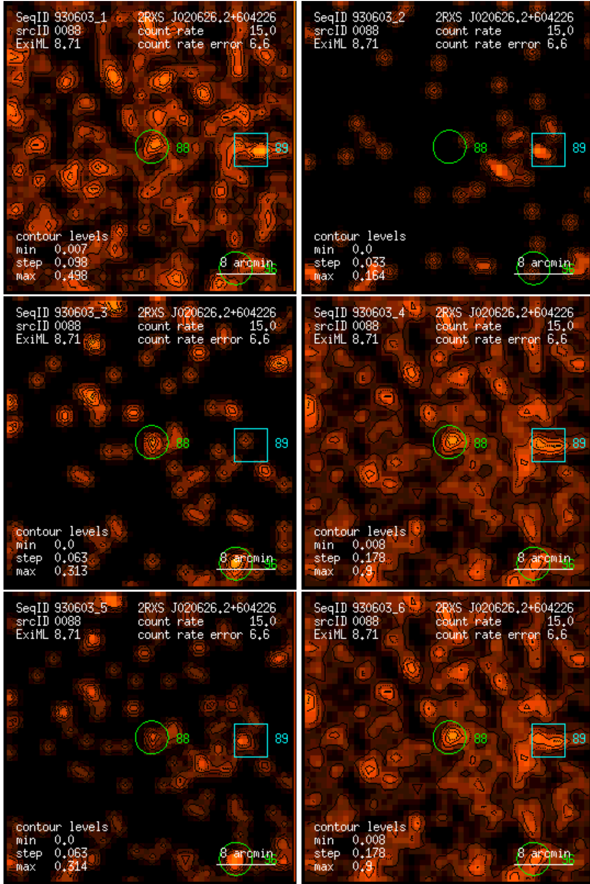
Figure 88: RASS 930603: detection 0088: band rate images, Gaussian filter: (1) PSPC channels 11 – 41, (2) 52 – 90, (3) 91 – 201, (4) 11 – 235, (5) 52 – 201, (6) 11 – 201. Broad band rates in counts/ks. Band rate contour levels in counts/ks/arcmin 2 .
