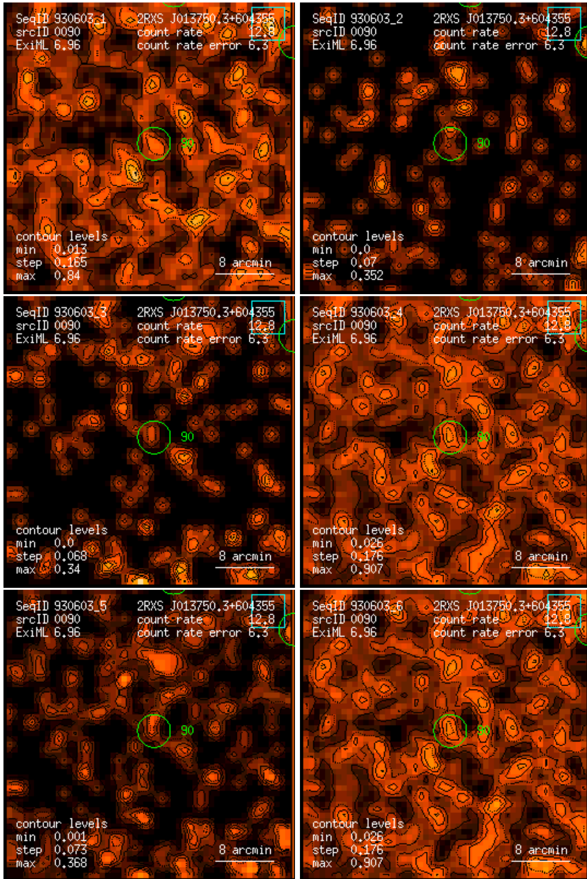
Figure 90: RASS 930603: detection 0090: band rate images, Gaussian filter: (1) PSPC channels 11 – 41, (2) 52 – 90, (3) 91 – 201, (4) 11 – 235, (5) 52 – 201, (6) 11 – 201. Broad band rates in counts/ks. Band rate contour levels in counts/ks/arcmin 2 .
