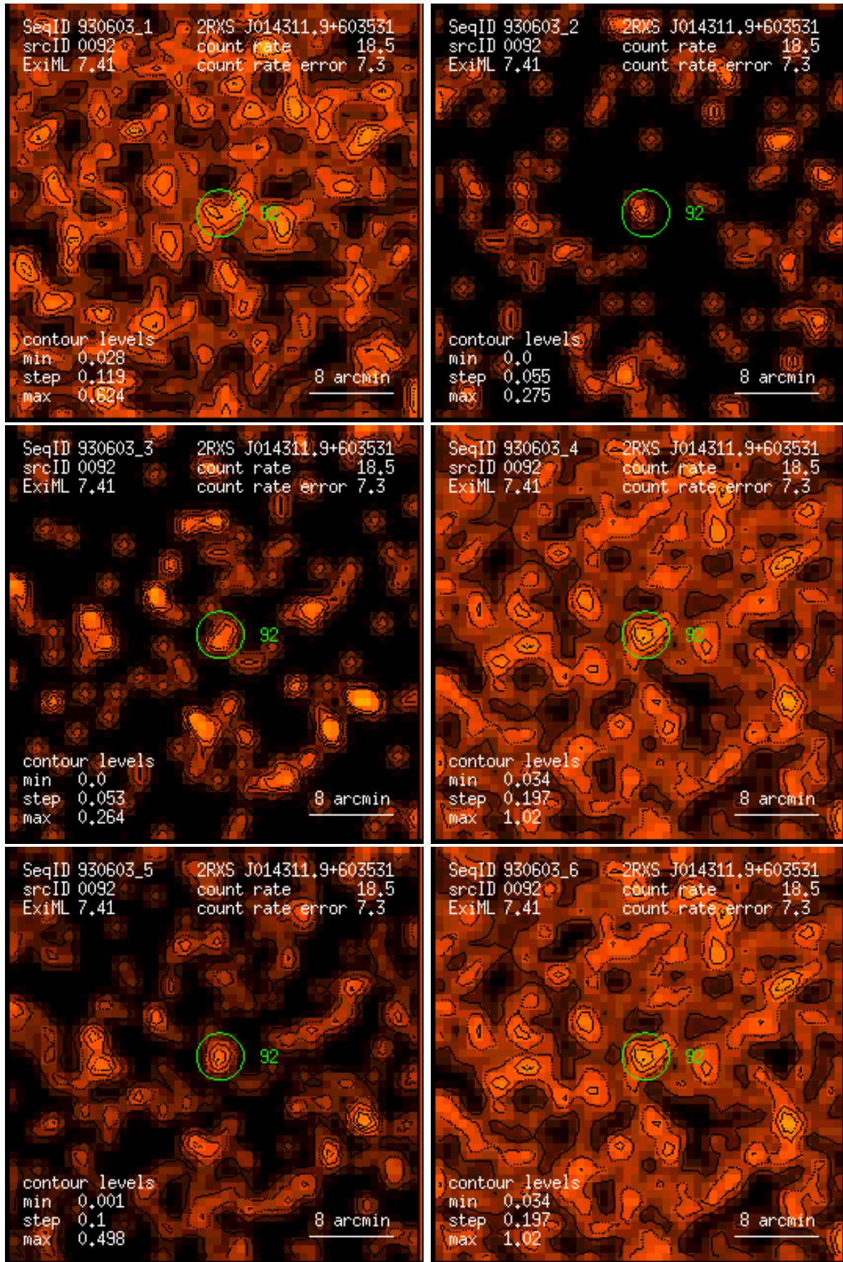
Figure 92: RASS 930603: detection 0092: band rate images, Gaussian filter: (1) PSPC channels 11 – 41, (2) 52 – 90, (3) 91 – 201, (4) 11 – 235, (5) 52 – 201, (6) 11 – 201. Broad band rates in counts/ks. Band rate contour levels in counts/ks/arcmin 2 .
