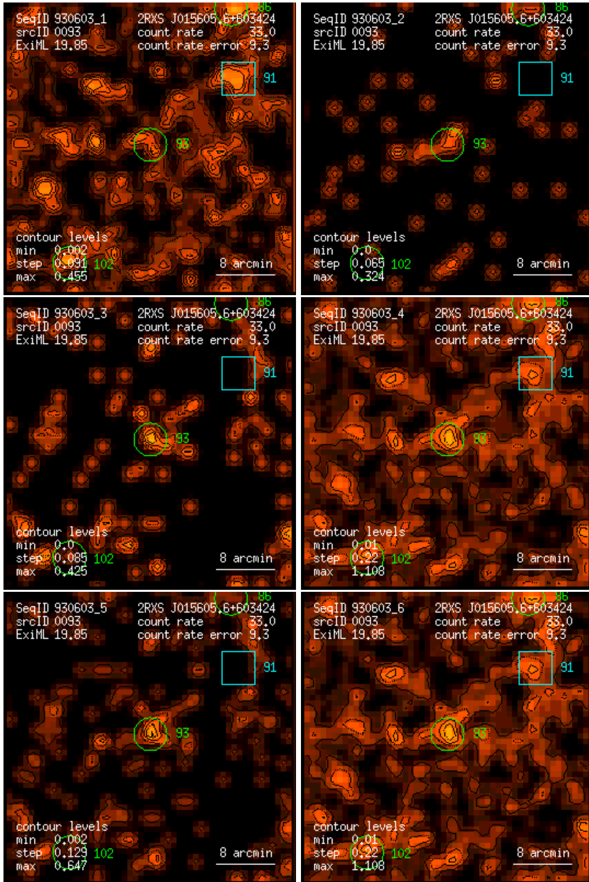
Figure 93: RASS 930603: detection 0093: band rate images, Gaussian filter: (1) PSPC channels 11 – 41, (2) 52 – 90, (3) 91 – 201, (4) 11 – 235, (5) 52 – 201, (6) 11 – 201. Broad band rates in counts/ks. Band rate contour levels in counts/ks/arcmin 2 .
