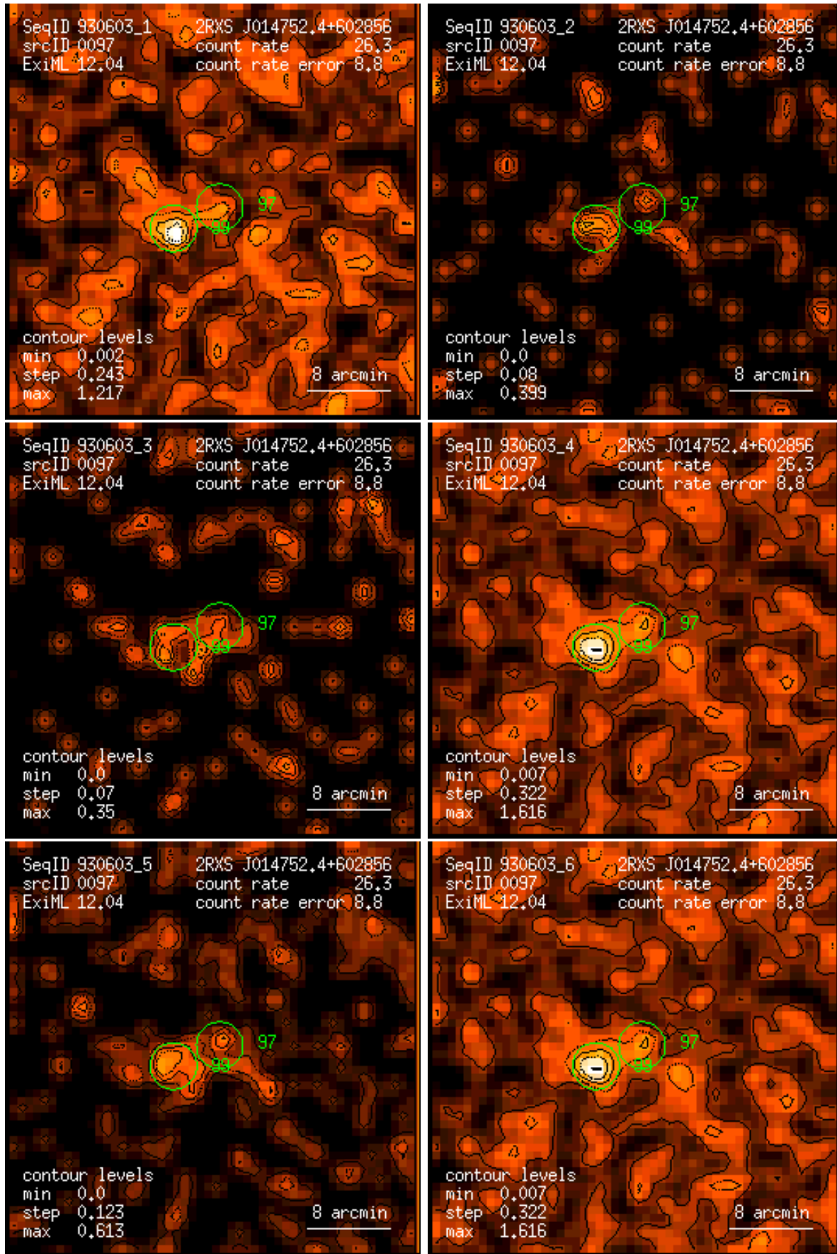
Figure 97: RASS 930603: detection 0097: band rate images, Gaussian filter: (1) PSPC channels 11 – 41, (2) 52 – 90, (3) 91 – 201, (4) 11 – 235, (5) 52 – 201, (6) 11 – 201. Broad band rates in counts/ks. Band rate contour levels in counts/ks/arcmin 2 .
