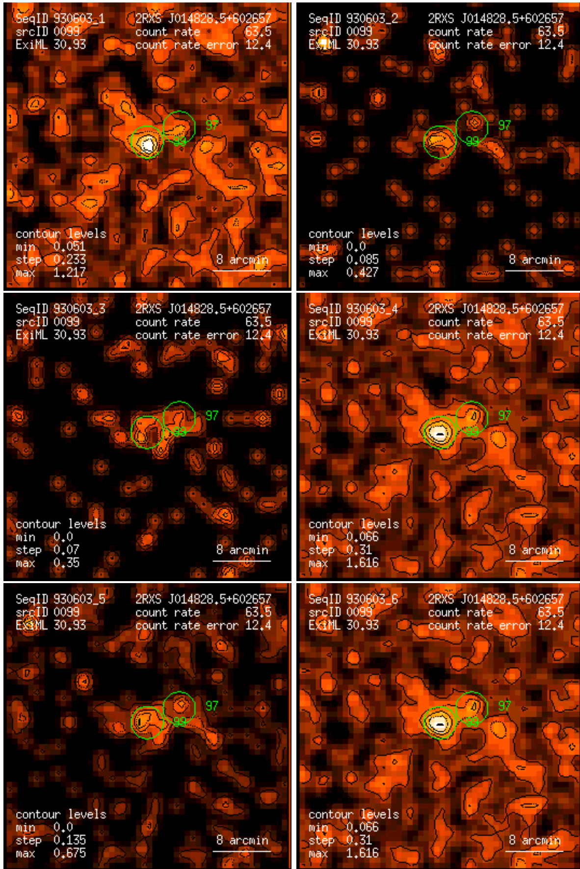
Figure 99: RASS 930603: detection 0099: band rate images, Gaussian filter: (1) PSPC channels 11 – 41, (2) 52 – 90, (3) 91 – 201, (4) 11 – 235, (5) 52 – 201, (6) 11 – 201. Broad band rates in counts/ks. Band rate contour levels in counts/ks/arcmin 2 .
