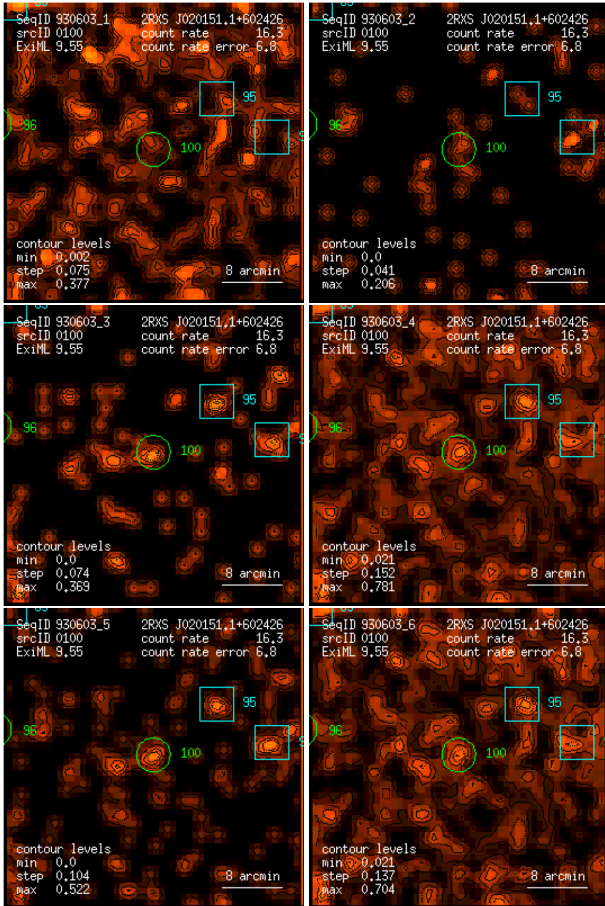
Figure 100: RASS 930603: detection 0100: band rate images, Gaussian filter: (1) PSPC channels 11 – 41, (2) 52 – 90, (3) 91 – 201, (4) 11 – 235, (5) 52 – 201, (6) 11 – 201. Broad band rates in counts/ks. Band rate contour levels in counts/ks/arcmin 2 .
