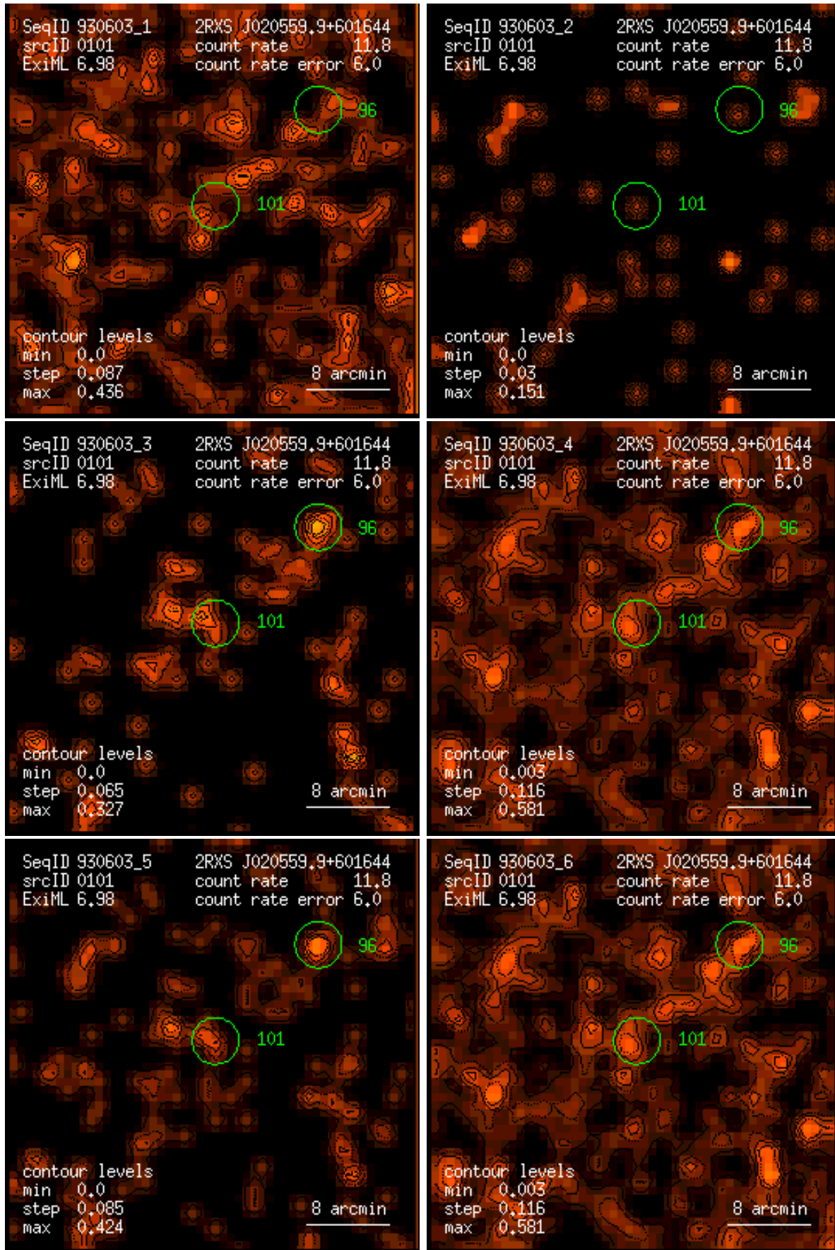
Figure 101: RASS 930603: detection 0101: band rate images, Gaussian filter: (1) PSPC channels 11 – 41, (2) 52 – 90, (3) 91 – 201, (4) 11 – 235, (5) 52 – 201, (6) 11 – 201. Broad band rates in counts/ks. Band rate contour levels in counts/ks/arcmin 2 .
