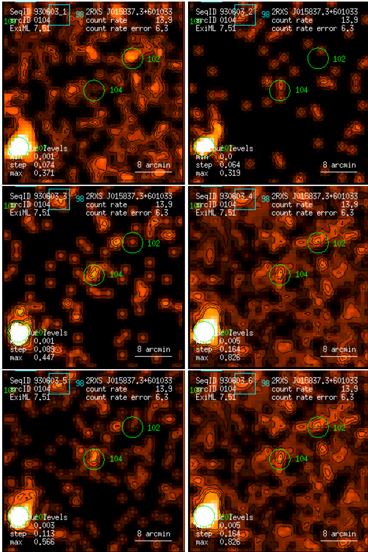
Figure 104: RASS 930603: detection 0104: band rate images, Gaussian filter: (1) PSPC channels 11 – 41, (2) 52 – 90, (3) 91 – 201, (4) 11 – 235, (5) 52 – 201, (6) 11 – 201. Broad band rates in counts/ks. Band rate contour levels in counts/ks/arcmin 2 .
