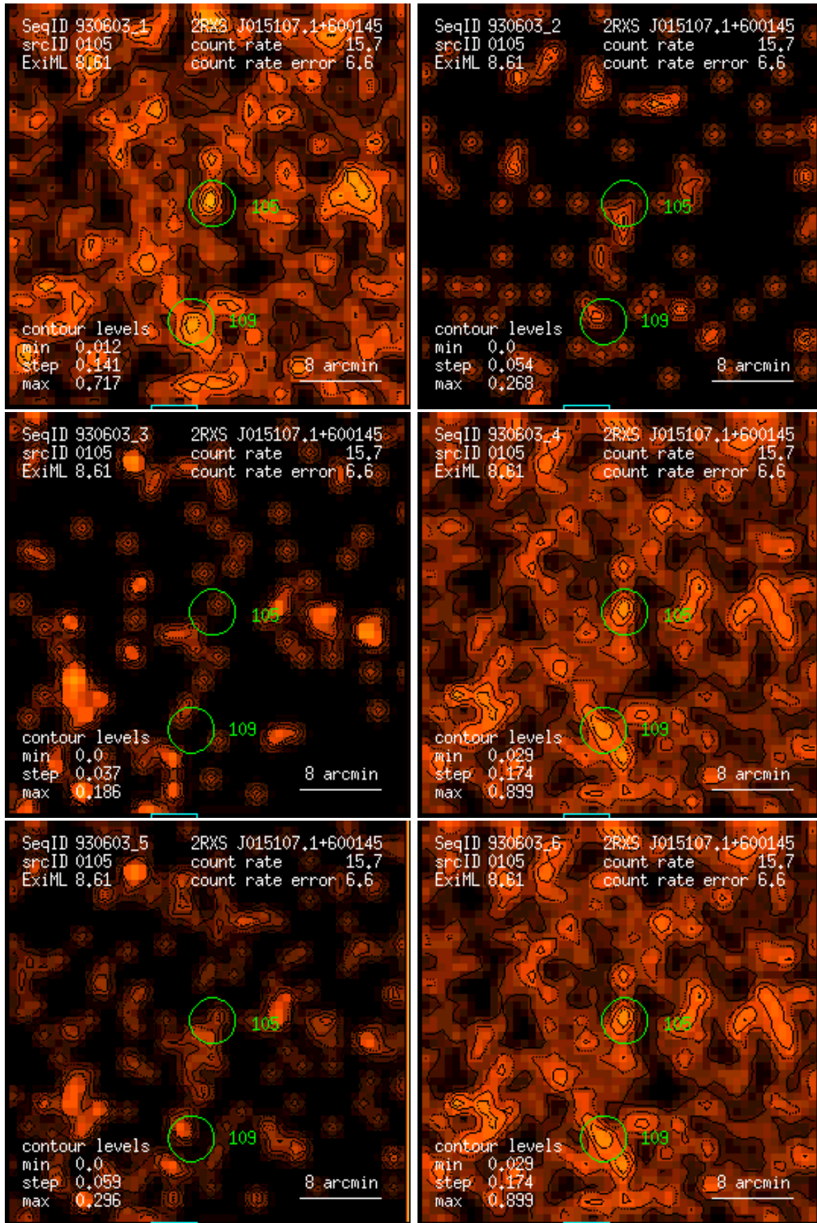
Figure 105: RASS 930603: detection 0105: band rate images, Gaussian filter: (1) PSPC channels 11 – 41, (2) 52 – 90, (3) 91 – 201, (4) 11 – 235, (5) 52 – 201, (6) 11 – 201. Broad band rates in counts/ks. Band rate contour levels in counts/ks/arcmin 2 .
