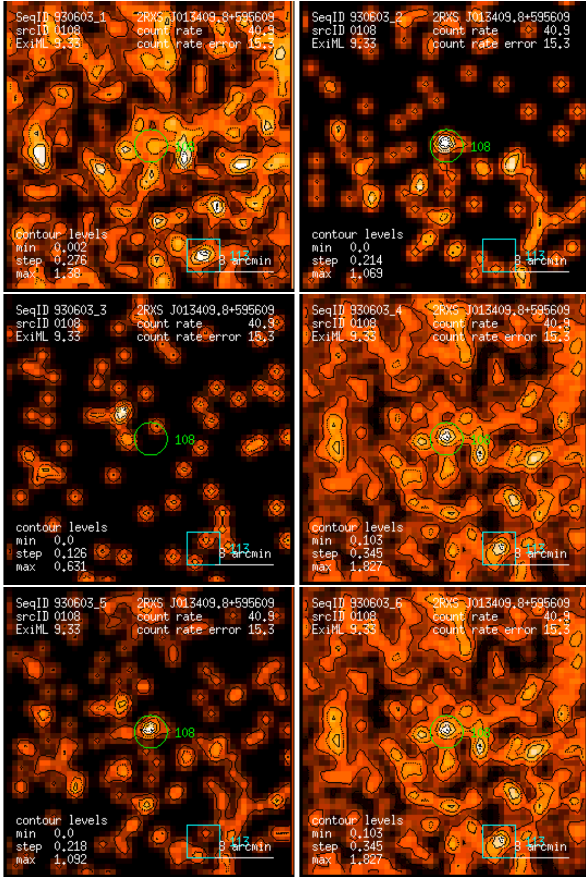
Figure 108: RASS 930603: detection 0108: band rate images, Gaussian filter: (1) PSPC channels 11 – 41, (2) 52 – 90, (3) 91 – 201, (4) 11 – 235, (5) 52 – 201, (6) 11 – 201. Broad band rates in counts/ks. Band rate contour levels in counts/ks/arcmin 2 .
