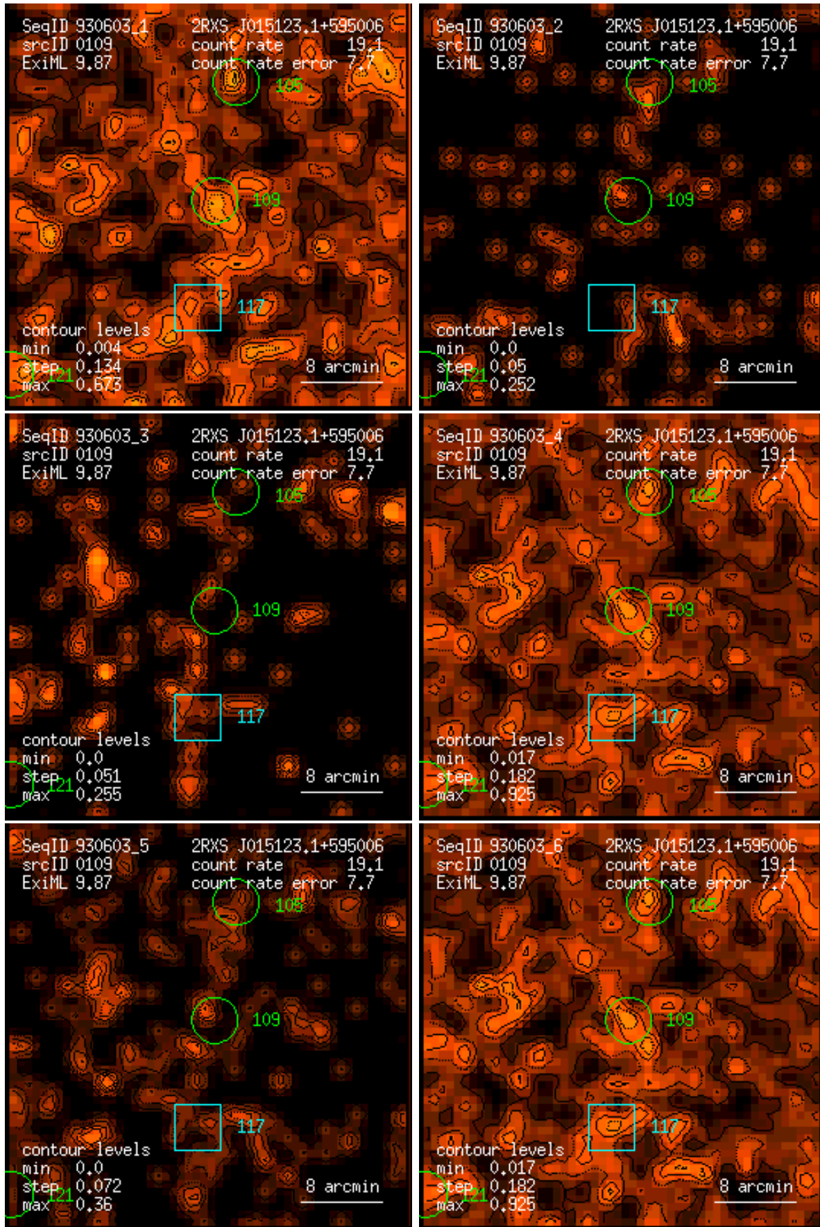
Figure 109: RASS 930603: detection 0109: band rate images, Gaussian filter: (1) PSPC channels 11 – 41, (2) 52 – 90, (3) 91 – 201, (4) 11 – 235, (5) 52 – 201, (6) 11 – 201. Broad band rates in counts/ks. Band rate contour levels in counts/ks/arcmin 2 .
