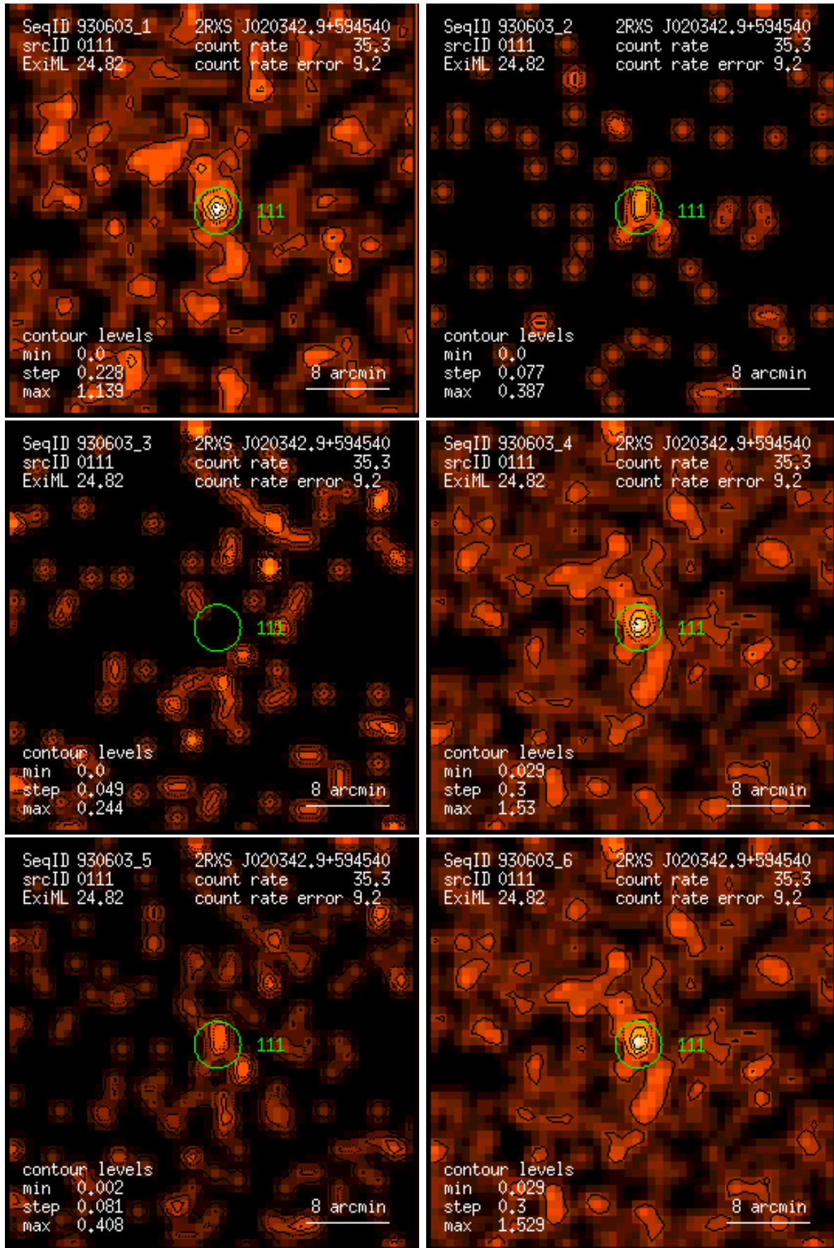
Figure 111: RASS 930603: detection 0111: band rate images, Gaussian filter: (1) PSPC channels 11 – 41, (2) 52 – 90, (3) 91 – 201, (4) 11 – 235, (5) 52 – 201, (6) 11 – 201. Broad band rates in counts/ks. Band rate contour levels in counts/ks/arcmin 2 .
