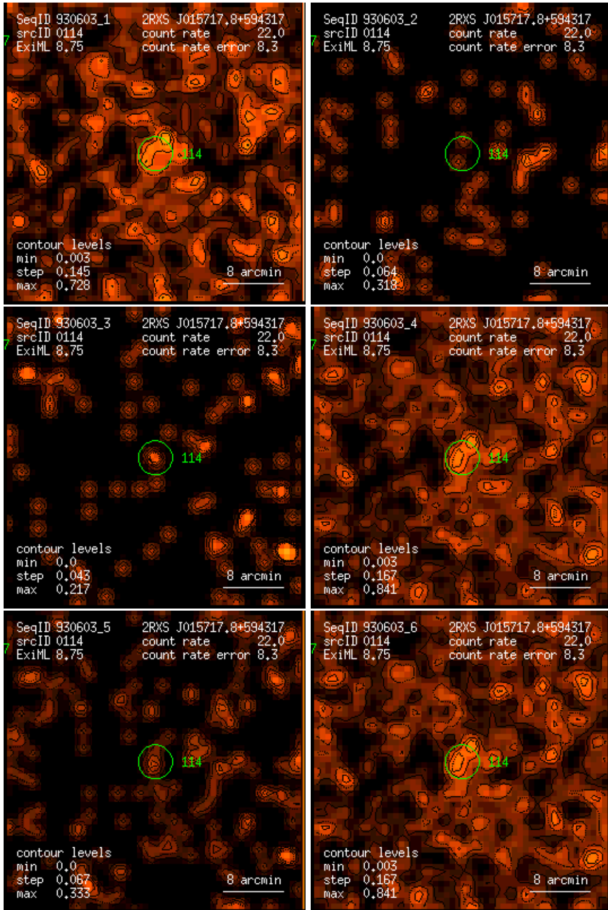
Figure 114: RASS 930603: detection 0114: band rate images, Gaussian filter: (1) PSPC channels 11 – 41, (2) 52 – 90, (3) 91 – 201, (4) 11 – 235, (5) 52 – 201, (6) 11 – 201. Broad band rates in counts/ks. Band rate contour levels in counts/ks/arcmin 2 .
