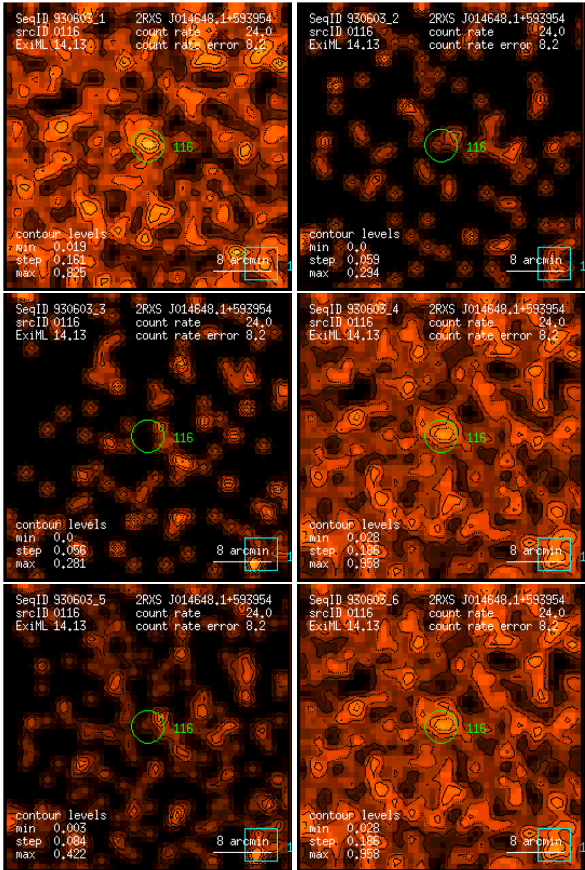
Figure 116: RASS 930603: detection 0116: band rate images, Gaussian filter: (1) PSPC channels 11 – 41, (2) 52 – 90, (3) 91 – 201, (4) 11 – 235, (5) 52 – 201, (6) 11 – 201. Broad band rates in counts/ks. Band rate contour levels in counts/ks/arcmin 2 .
