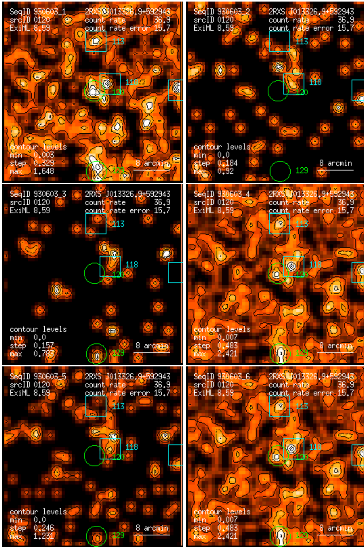
Figure 120: RASS 930603: detection 0120: band rate images, Gaussian filter: (1) PSPC channels 11 – 41, (2) 52 – 90, (3) 91 – 201, (4) 11 – 235, (5) 52 – 201, (6) 11 – 201. Broad band rates in counts/ks. Band rate contour levels in counts/ks/arcmin 2 .
