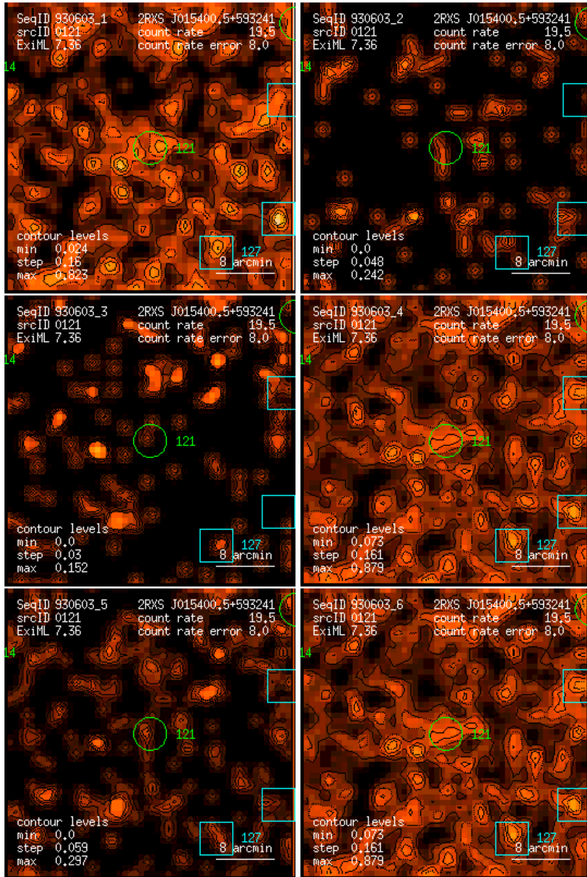
Figure 121: RASS 930603: detection 0121: band rate images, Gaussian filter: (1) PSPC channels 11 – 41, (2) 52 – 90, (3) 91 – 201, (4) 11 – 235, (5) 52 – 201, (6) 11 – 201. Broad band rates in counts/ks. Band rate contour levels in counts/ks/arcmin 2 .
